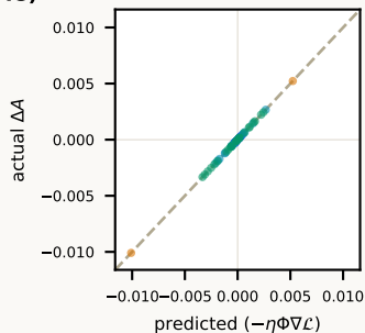
(f) Kernel prediction r = 1.000
