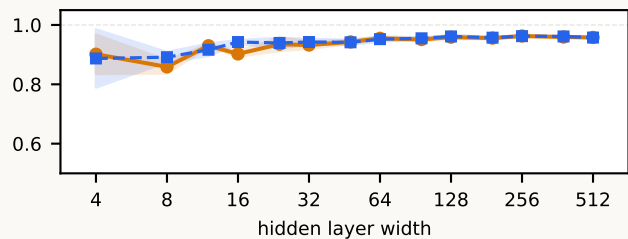
(k) Width sweep (depth = 3)
