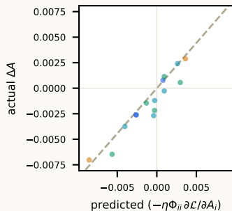
(c) Diagonal approximation r = 0.952
