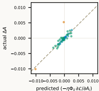
(g) Diagonal approximation r = 0.892
