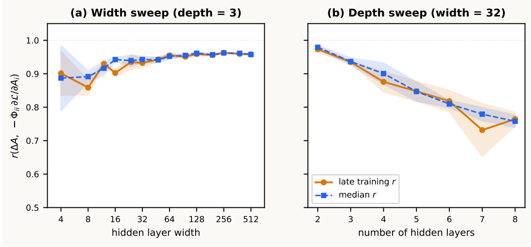
Figure 2: Width and depth control the accuracy of the diagonal approximation in this toy setting. Pearson r between actual \Delta A and -\Phi_{ii} \partial \mathcal{L} / \partial A_i . (a) Hidden-layer width on a log 2 scale at fixed depth 3. (b) Number of hidden layers at fixed width 32. Orange shows the mean correlation over the final five diagnostics; blue shows the median correlation over training. Dead ReLU neurons excluded. Shaded regions: \pm 1 s.d. across seeds.
