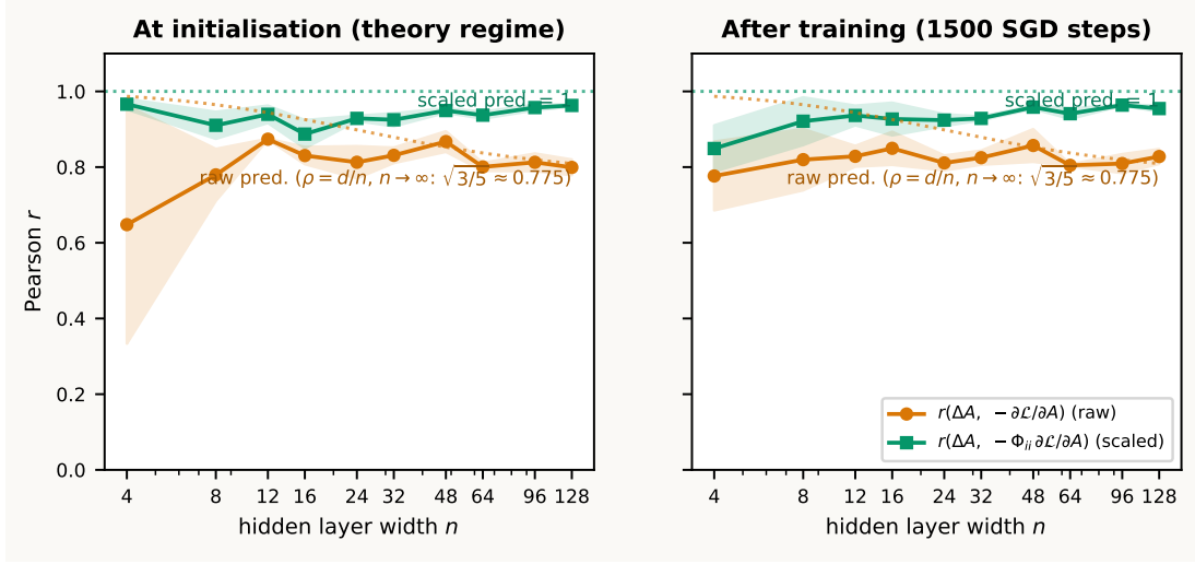
Figure 4: Width sweep at fixed depth ( D = 3 , 3 seeds). Pearson r between actual \Delta A and the gradient signal, plotted against hidden-layer width n on a log scale. Orange: raw gradient -\partial\mathcal{L}/\partial A . Green: gradient scaled by \Phi_{ii}^{(\ell)} . Left: averages over the first 3 diagnostics (initialisation regime). Right: averages over the last 5 diagnostics (after 1500 SGD steps). Dotted curves mark the leading-order predictions: r_{\text{raw}}(3, d/n) from Eq. 9 (orange; descending to \sqrt{3/5} \approx 0.775 at large n ) and r_{\text{scaled}} \approx 1 (green).
