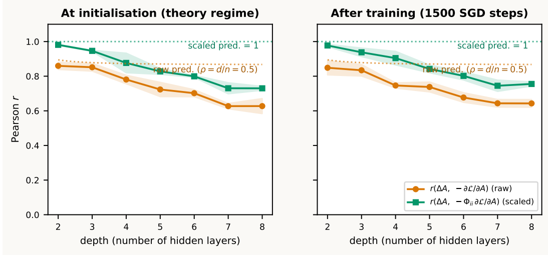
Figure 3: Depth sweep at fixed width ( n = 32 , 3 seeds). Pearson r between actual \Delta\mathbf{A} and the gradient signal, plotted against network depth. Orange: raw gradient -\partial\mathcal{L}/\partial\mathbf{A} . Green: gradient scaled by \Phi_{ii}^{(\ell)} . Left panel averages the first 3 diagnostics (initialisation regime); right panel averages the last 5 diagnostics (after 1500 SGD steps). Dotted curves mark the leading-order predictions: r_{\text{raw}}(D, \rho=0.5) from Eq. 9 (orange; nearly flat near 0.87–0.89 across this depth range because \rho = d/n = 16/32 ) and r_{\text{scaled}} \approx 1 (green).
