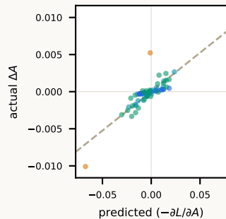
-dL/dA (raw) r = 0.832
