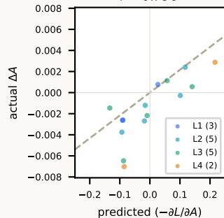
-dL/dA (raw) r = 0.796
