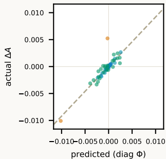
Eq. 5 (diagonal) r = 0.892
