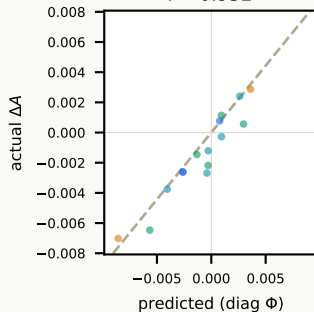
Eq. 5 (diagonal) r = 0.952
