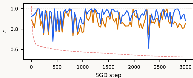
(i) Training dynamics (width = 8)
