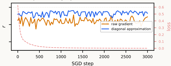
(j) Training dynamics (width = 48)
