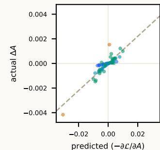
-d\mathcal{L}/dA (raw) r = 0.890
