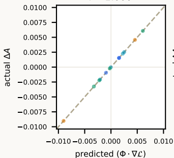
Kernel prediction r = 1.000
