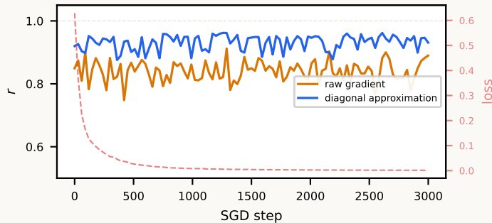
Training dynamics (width=48)
