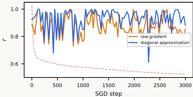
Training dynamics (width=8)
