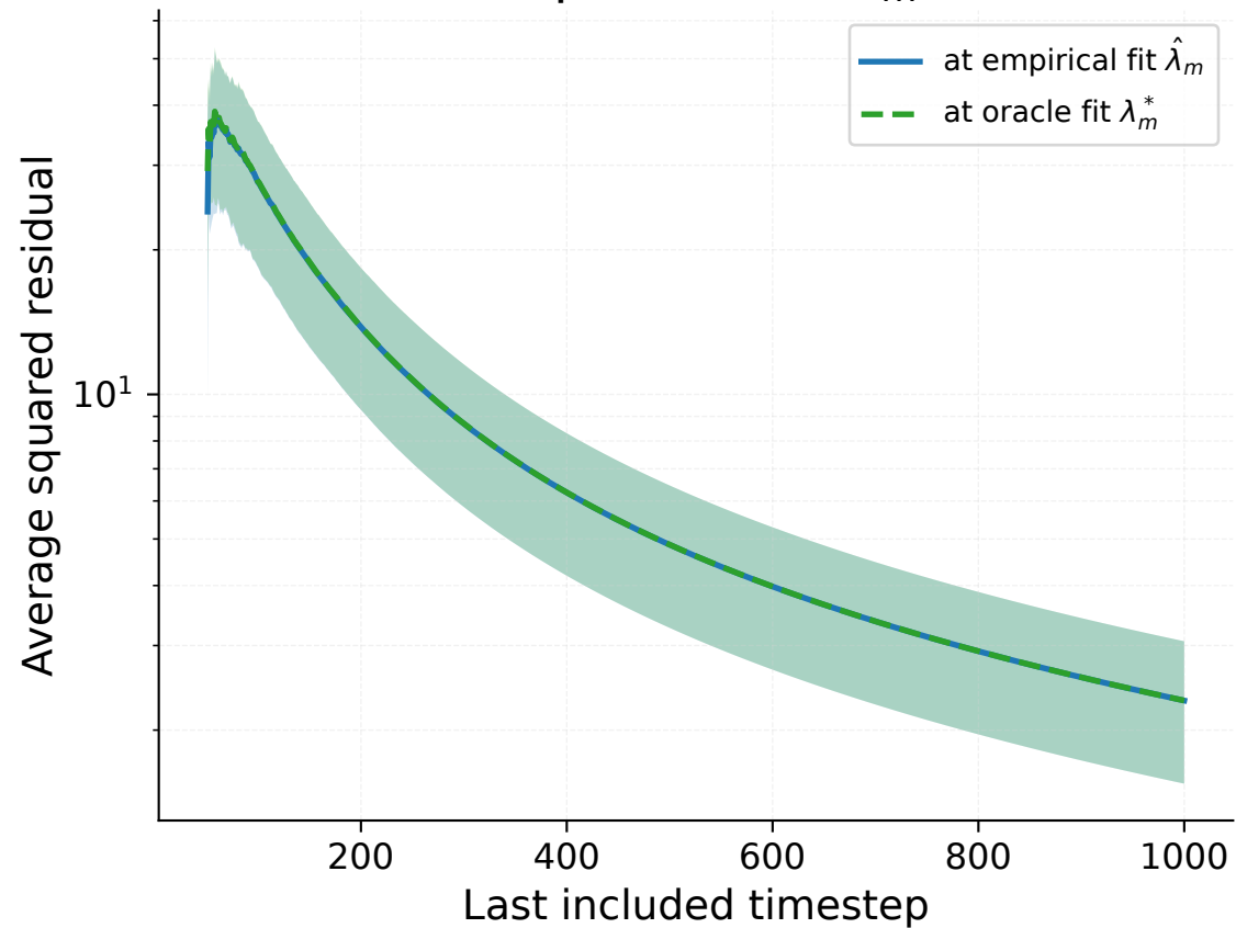
Empirical loss \hat{E}_m
