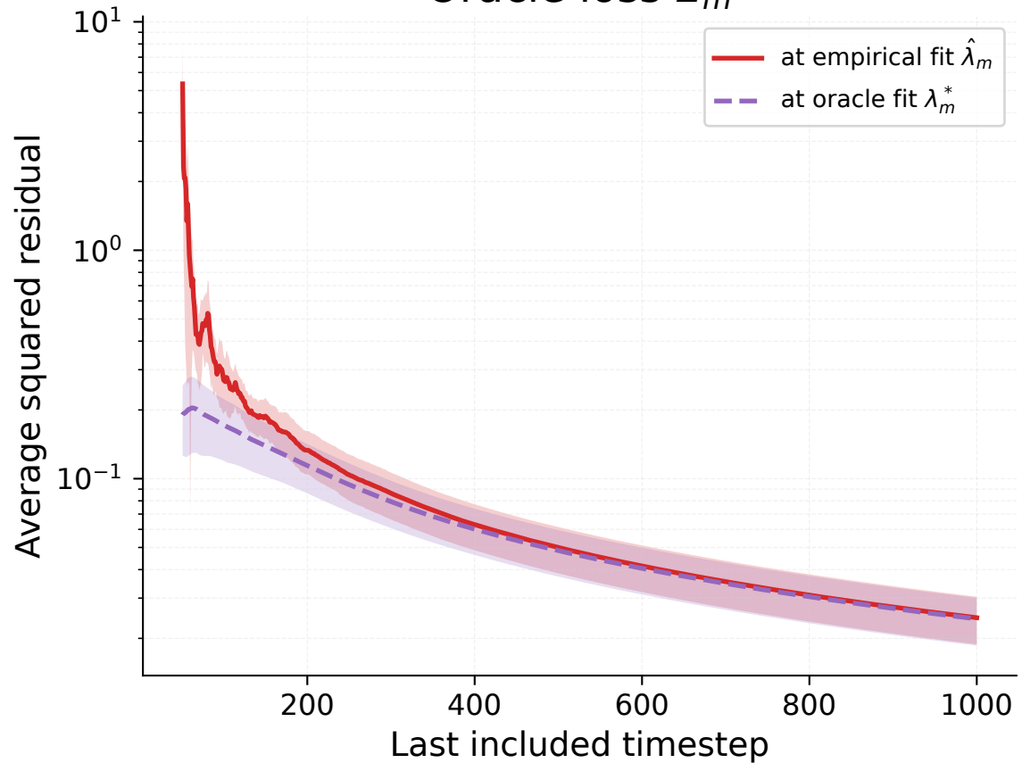
Oracle loss E_m
