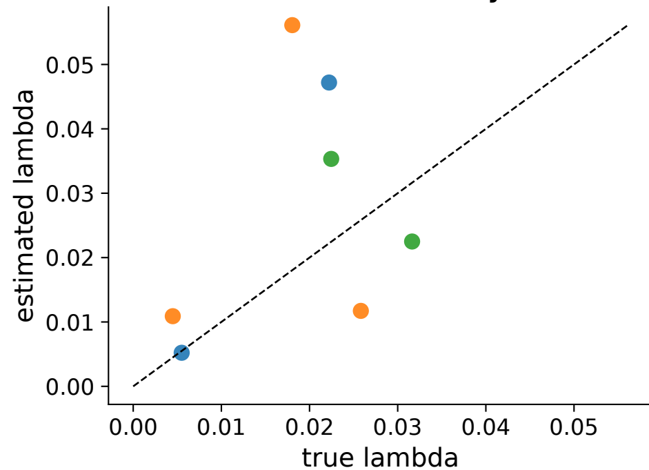
Scale Recovery
