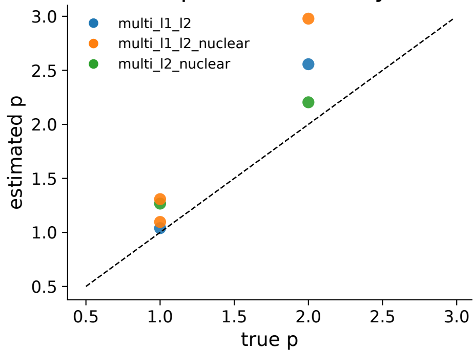
Exponent Recovery
