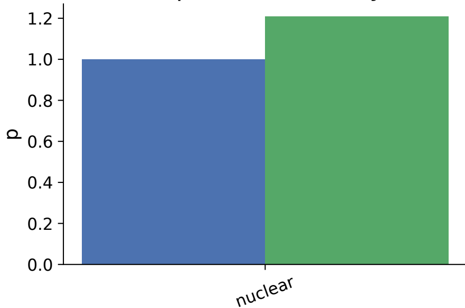
Exponent Recovery
