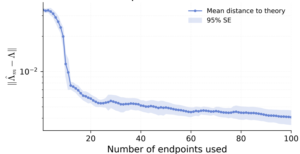
Multi-endpoint estimation error
