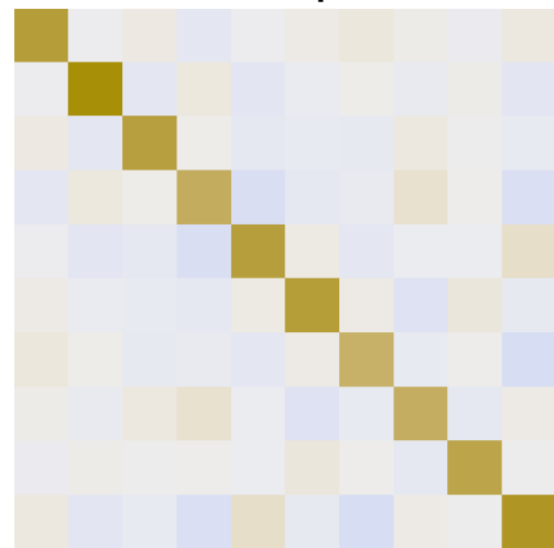
B Multi-endpoint \hat{\Lambda}
