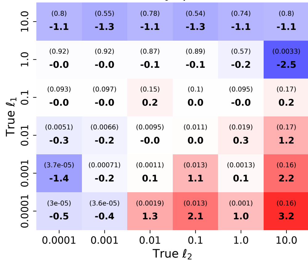
\ell_1 Recovery ( \beta = 0.001 )
