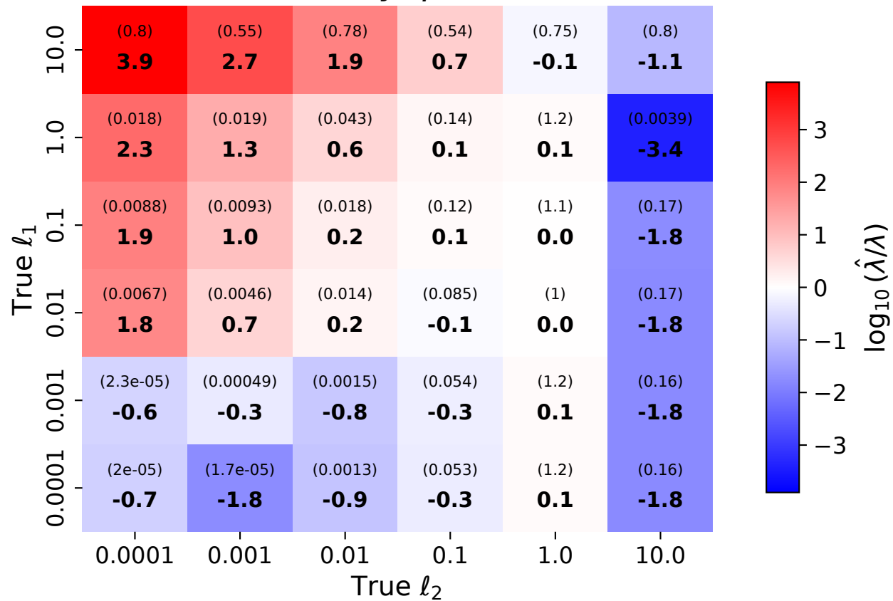
\ell_2 Recovery ( \beta = 0.001 )
