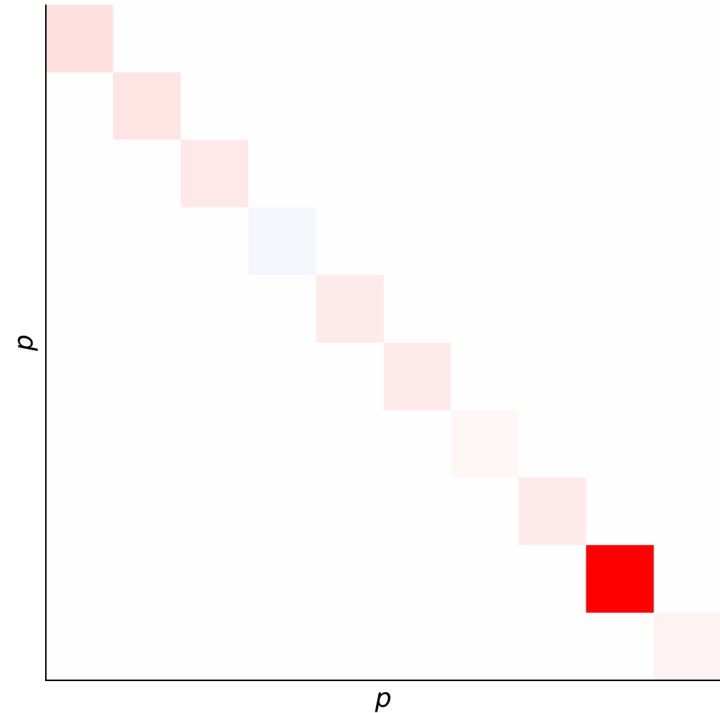
Estimated \hat{\Lambda}
