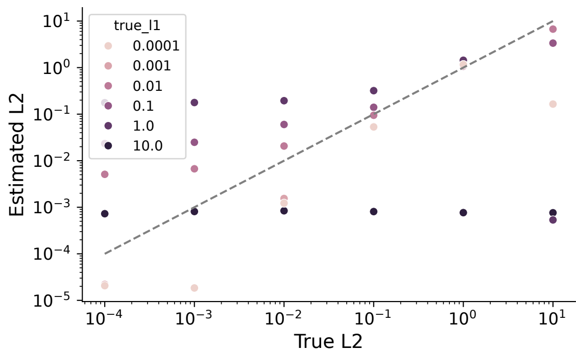
Estimated vs True L2 Smoothing: \beta = 0.0001
