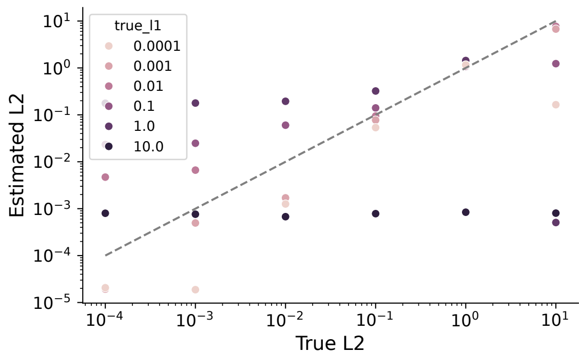
Estimated vs True L2 Smoothing: \beta = 1e - 05
