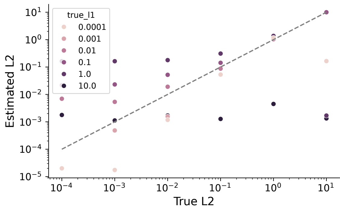
Estimated vs True L2 Smoothing: \beta = 0.001
