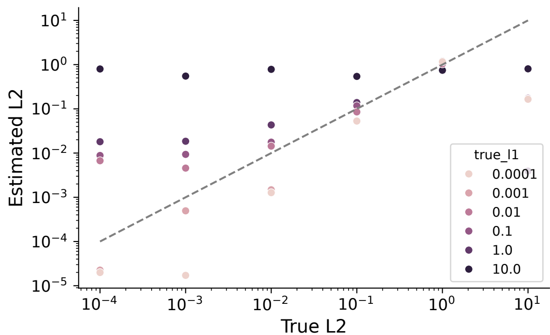
Estimated vs True L2 Smoothing: \beta = 0.01
