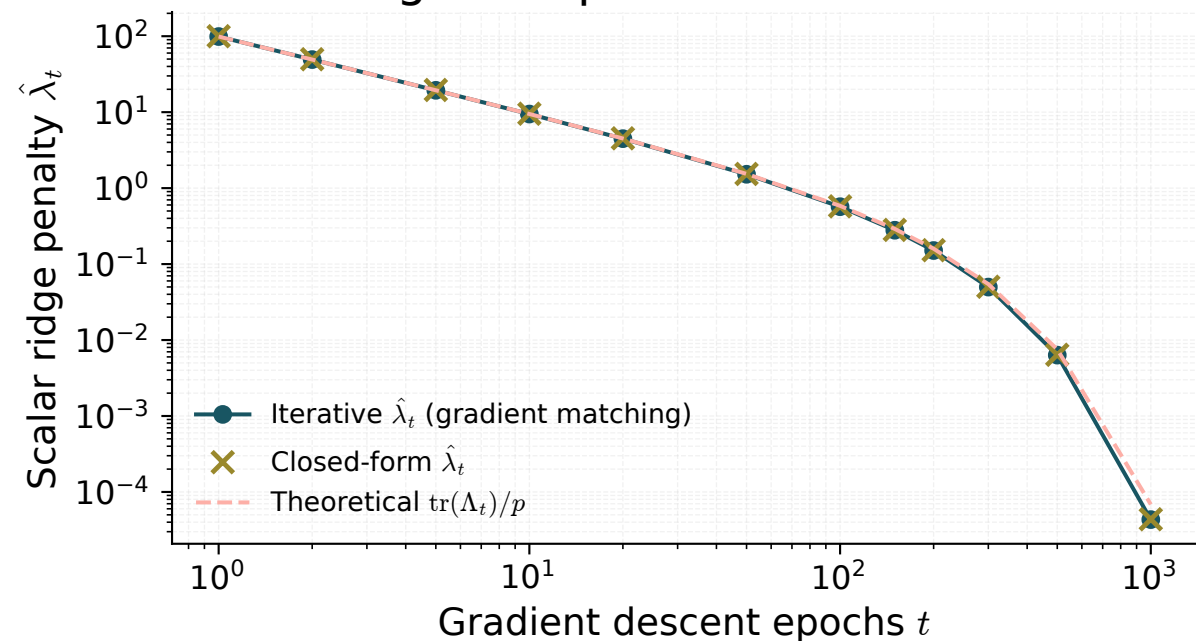
Heuristic single-endpoint estimator over training
