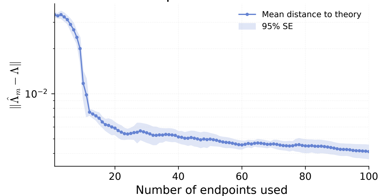
Multi-endpoint estimation error
