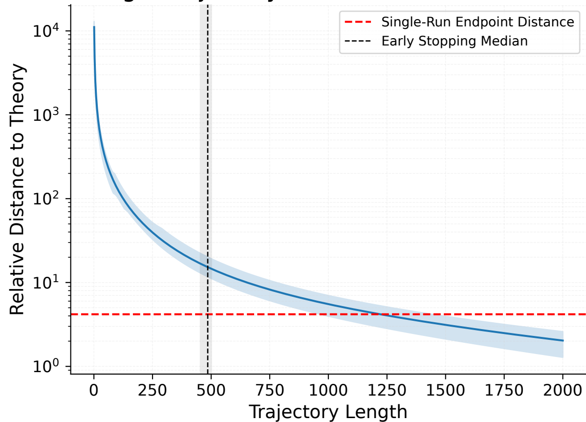
Single-trajectory fit: median over 10 runs
