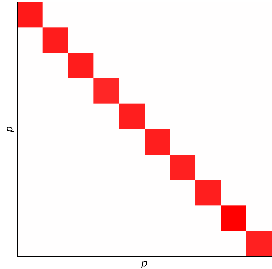
Estimated \hat{\Lambda}
