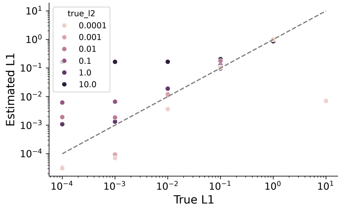
Estimated vs True L1 Smoothing: \beta = 0.01
