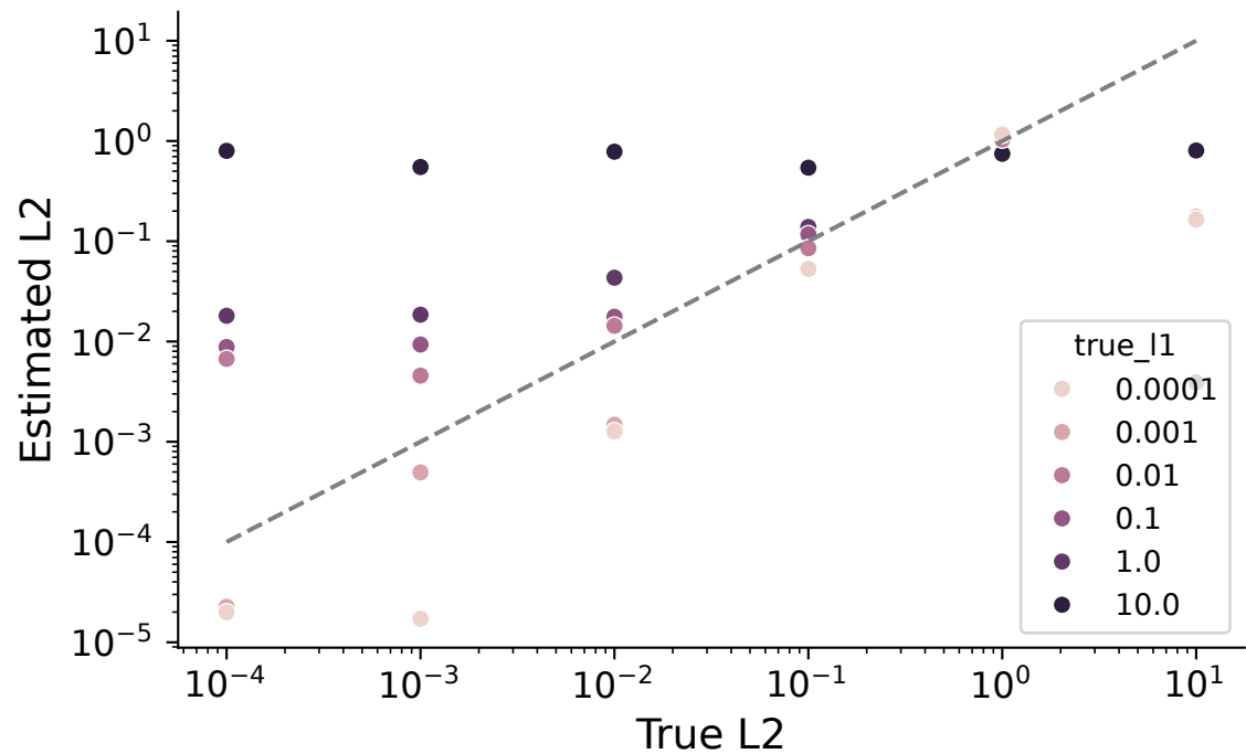
Estimated vs True L2 Smoothing: \beta = 0.01
