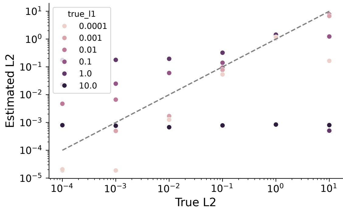
Estimated vs True L2 Smoothing: \beta = 1e - 05
