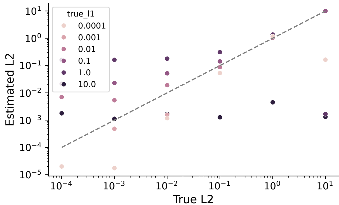
Estimated vs True L2 Smoothing: \beta = 0.001
