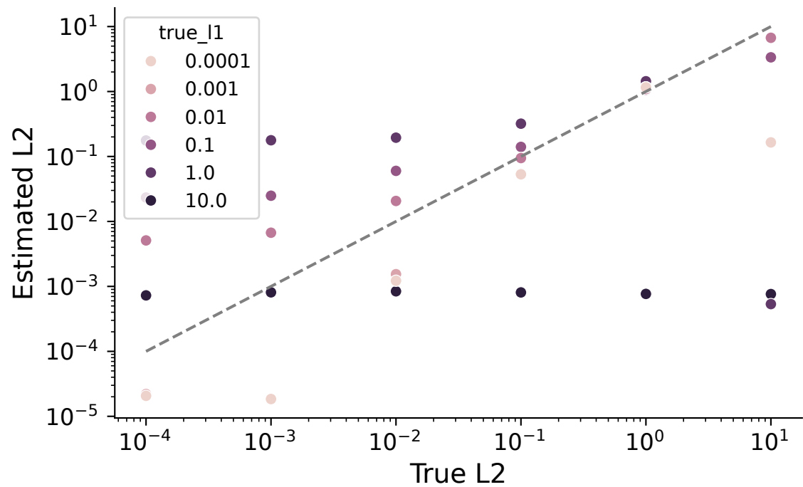
Estimated vs True L2 Smoothing: \beta = 0.0001
