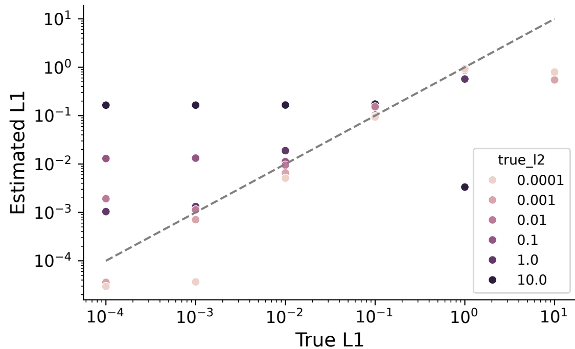
Estimated vs True L1 Smoothing: \beta = 0.01
