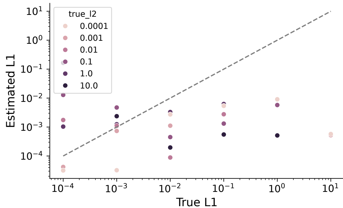
Estimated vs True L1 Smoothing: \beta = 1e - 05
