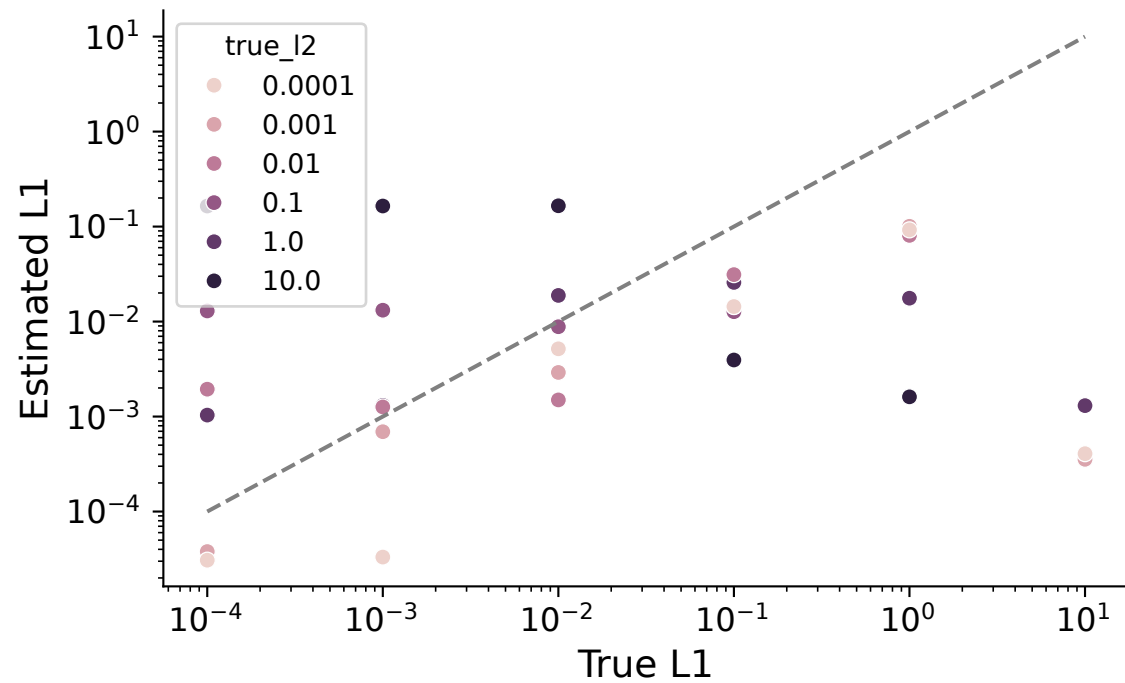
Estimated vs True L1 Smoothing: \beta = 0.001
