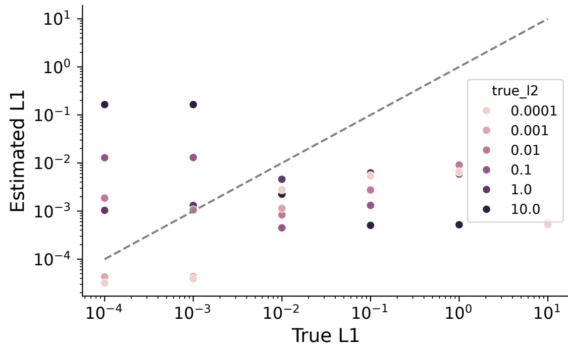
Estimated vs True L1 Smoothing: \beta = 0.0001
