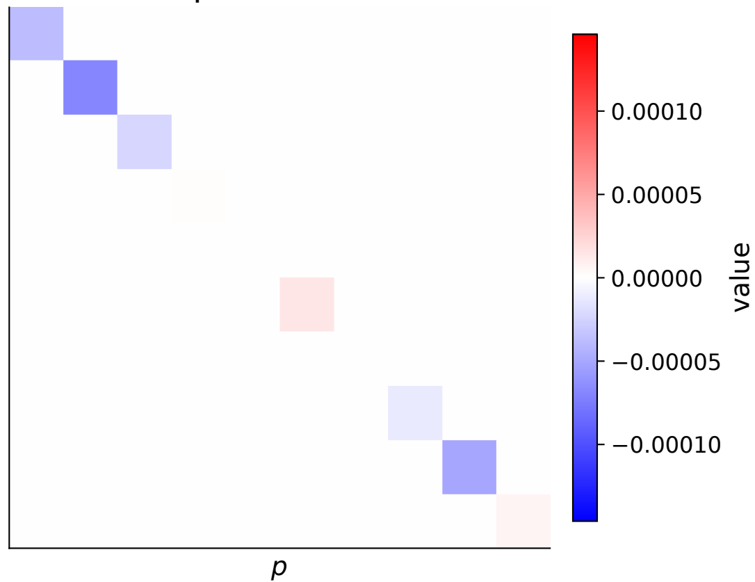
1-endpoint SGD-vs-GD fit 10-endpoint reference \Lambda
