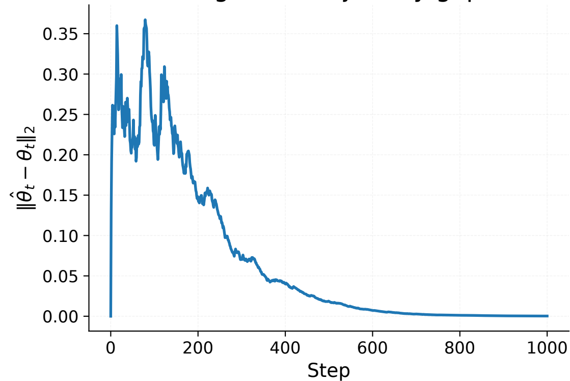
Single-run trajectory gap
