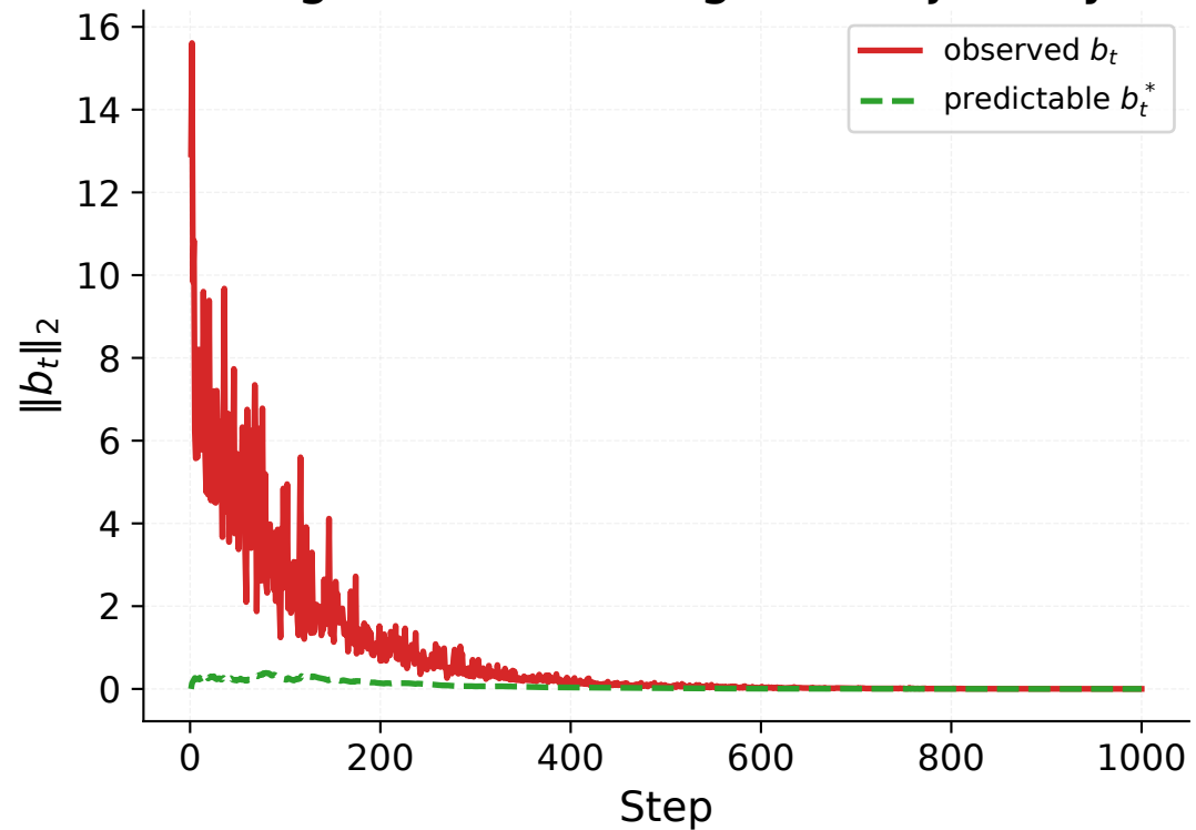
Target norms along the trajectory
