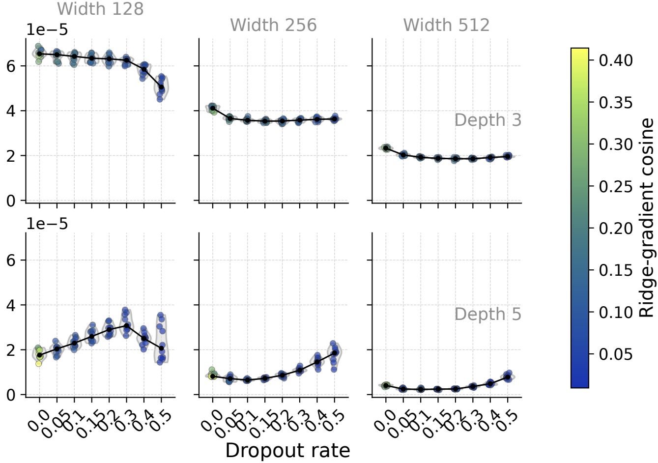
Closed-form ridge penalty \hat{\lambda}
