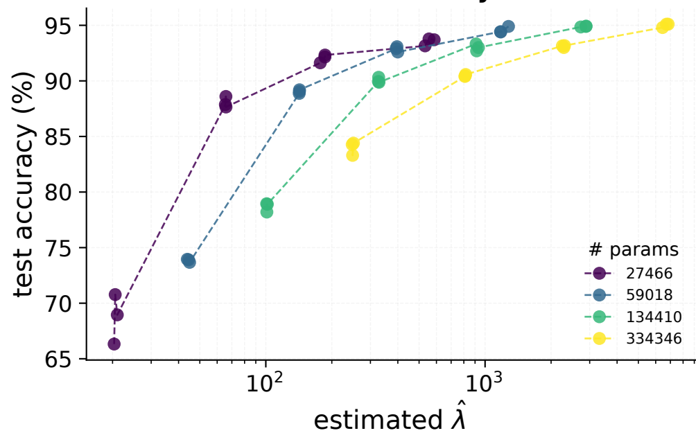
(b) Test accuracy vs \hat{\lambda}
