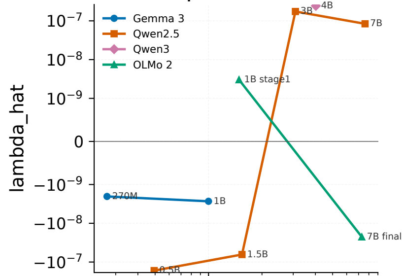
Embedding / LM head
