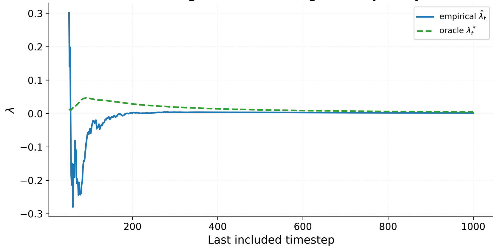
Scalar ridge estimate along one trajectory
