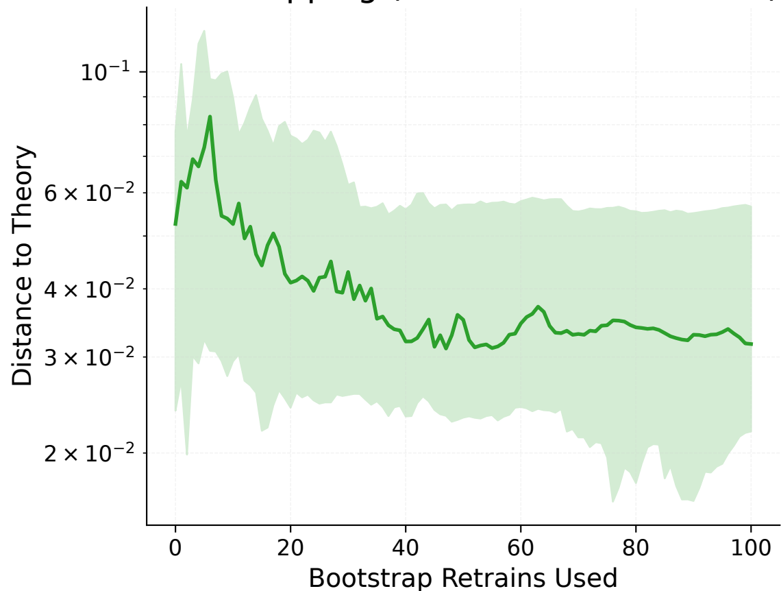
Bootstrapping (median over 10 seeds)
