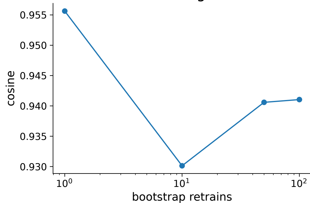
Gradient Alignment
