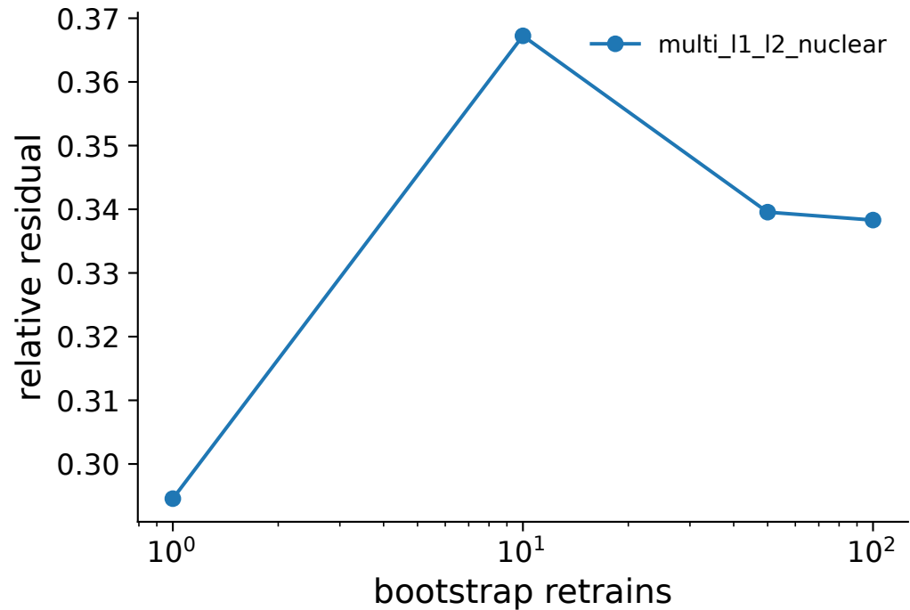
Relative Residual
