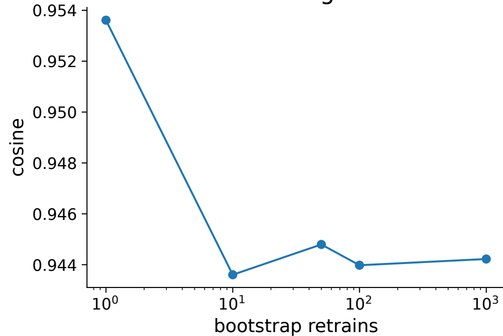
Gradient Alignment
