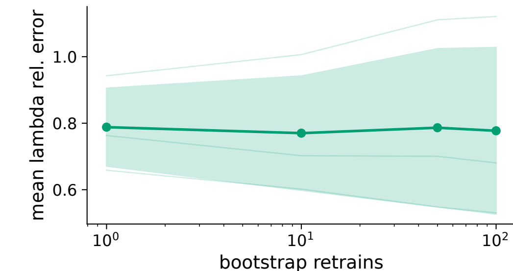
Scale Error
