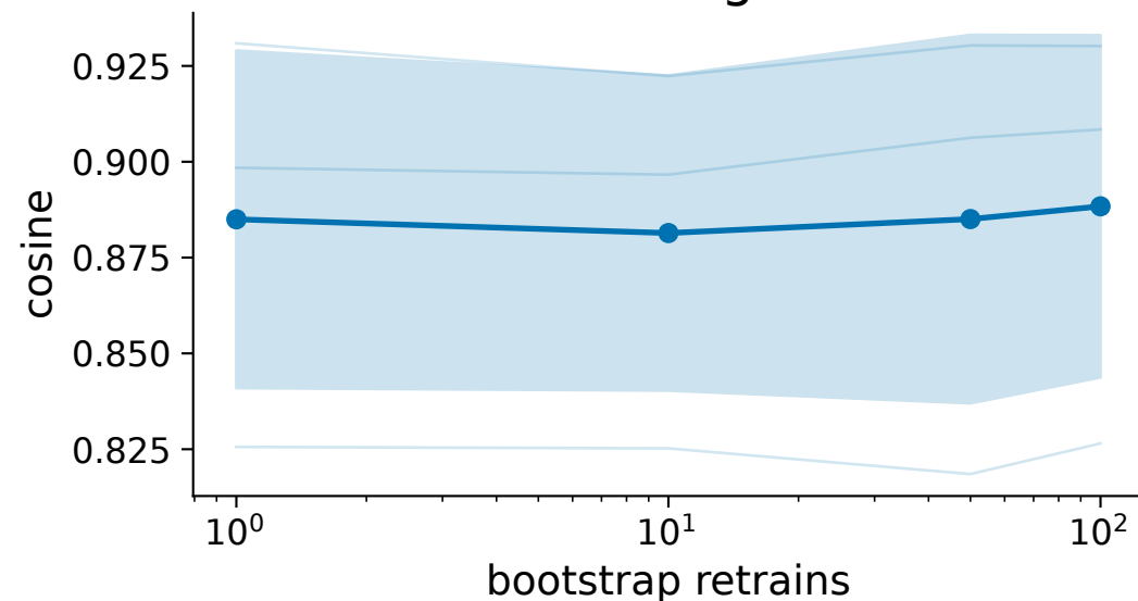
Scale Error
