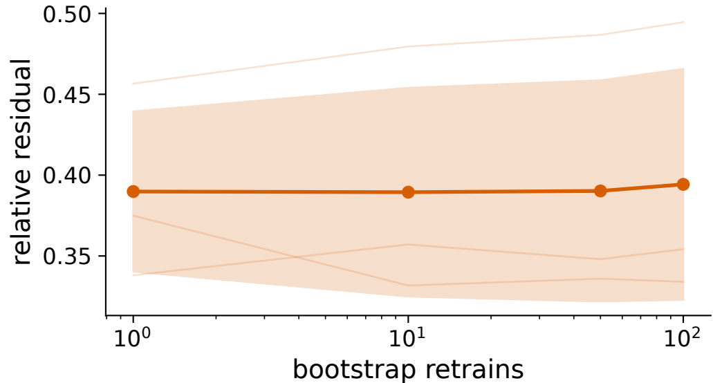
Relative Residual
