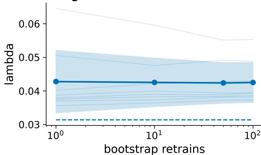
Single Active Elementwise L2
