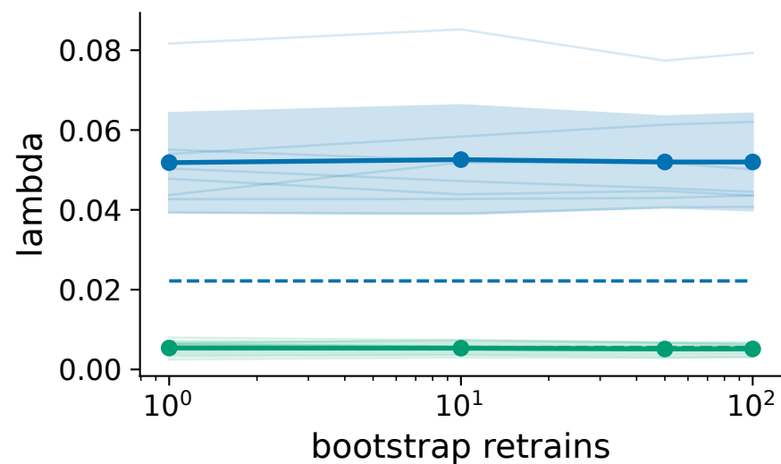
Mixed Elementwise L1 + L2
