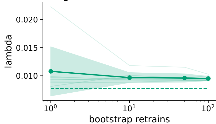
Single Active Elementwise L1
