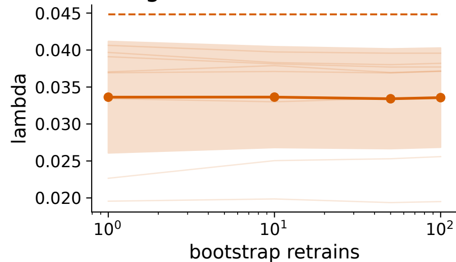
Single Active Nuclear Norm
