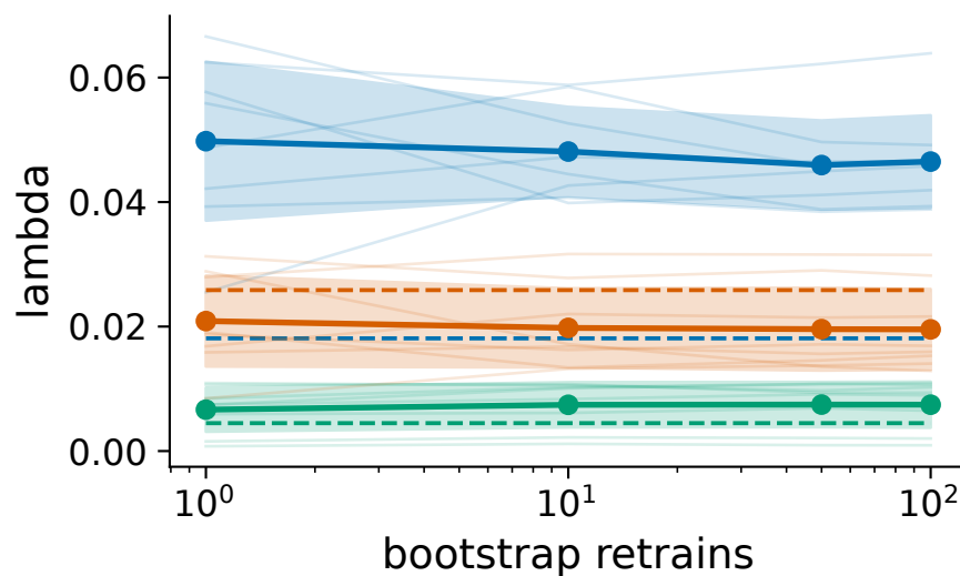
Mixed Elementwise L1 + L2 + Nuclear
