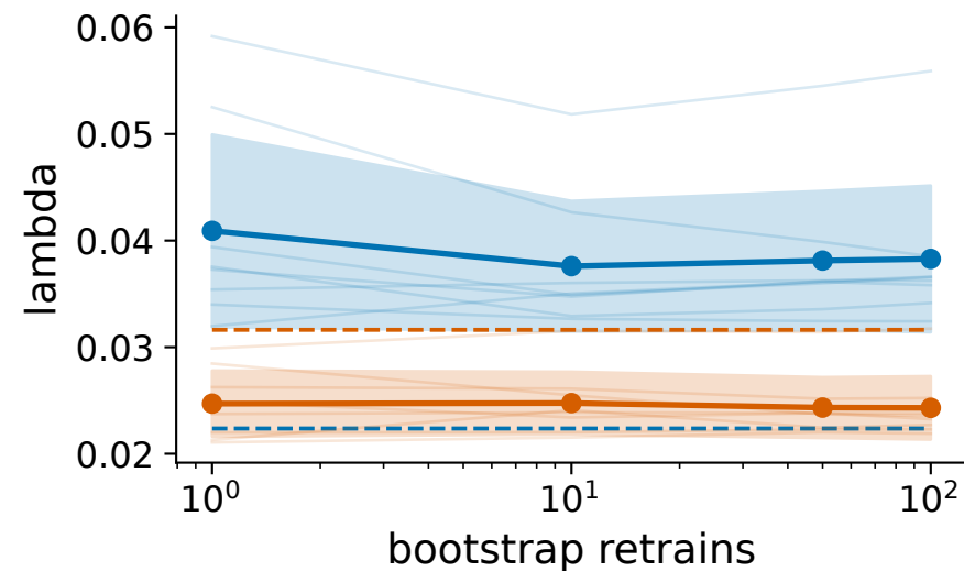
Mixed Elementwise L2 + Nuclear
