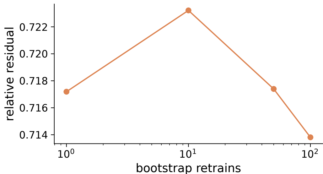
Relative Residual
