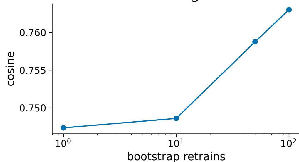
Scale Trajectories
