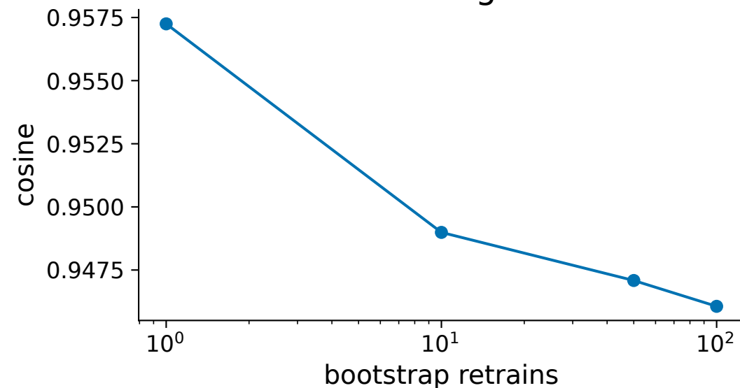
Scale Trajectories
