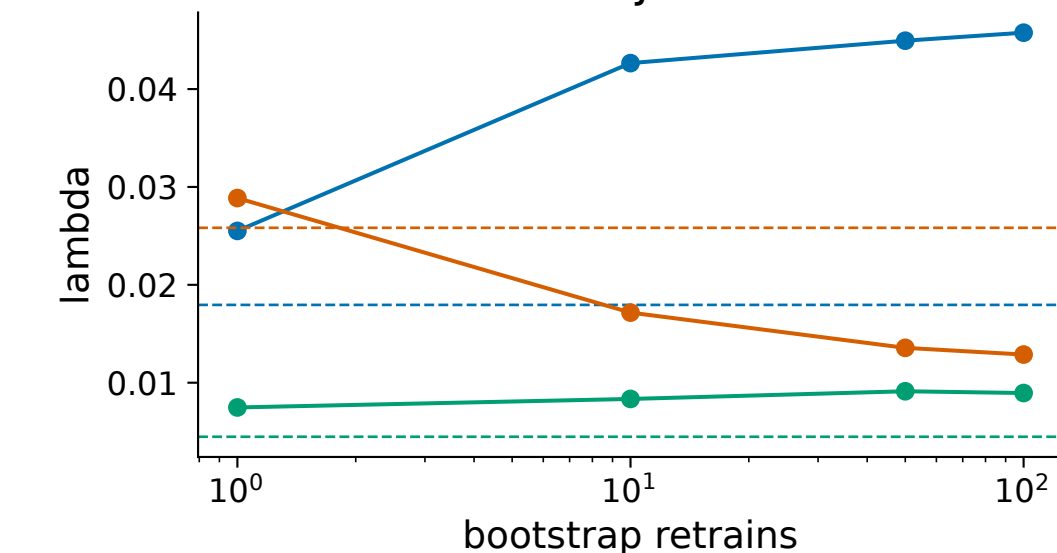
Scale Trajectories
