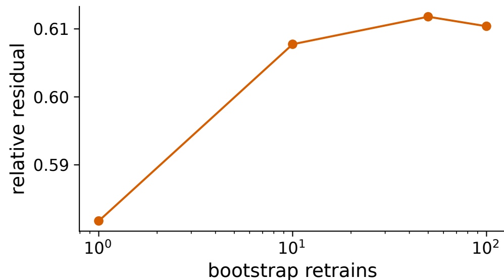
Relative Residual
