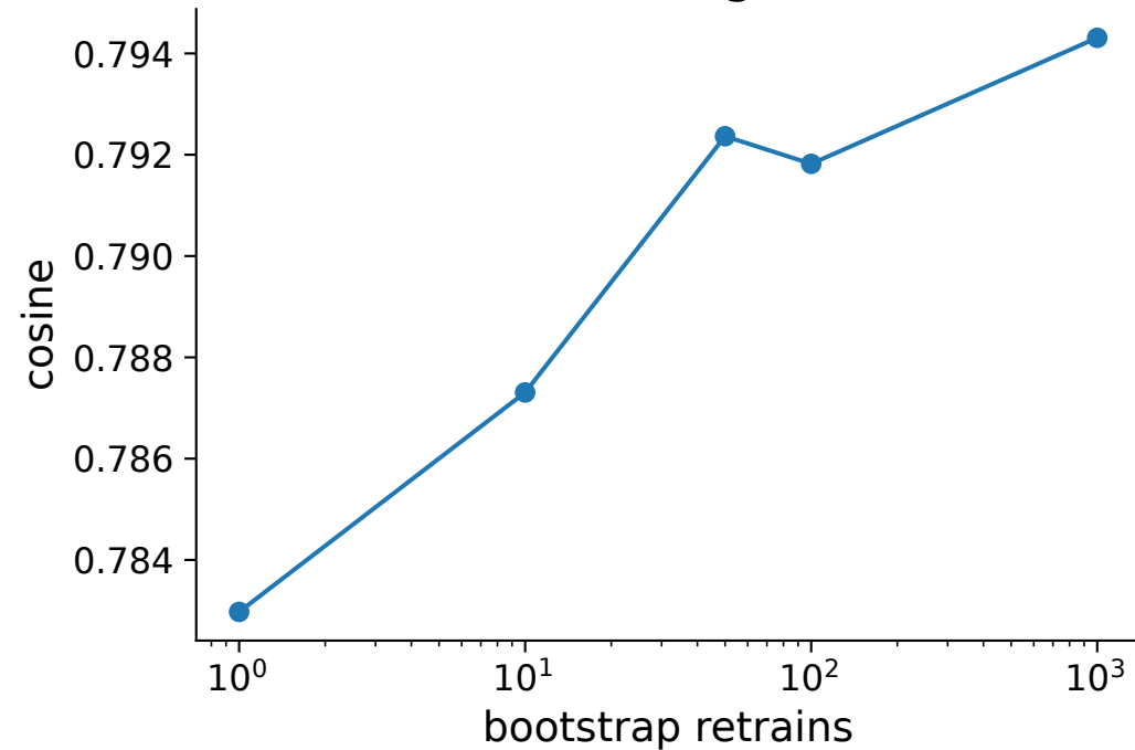
Gradient Alignment
