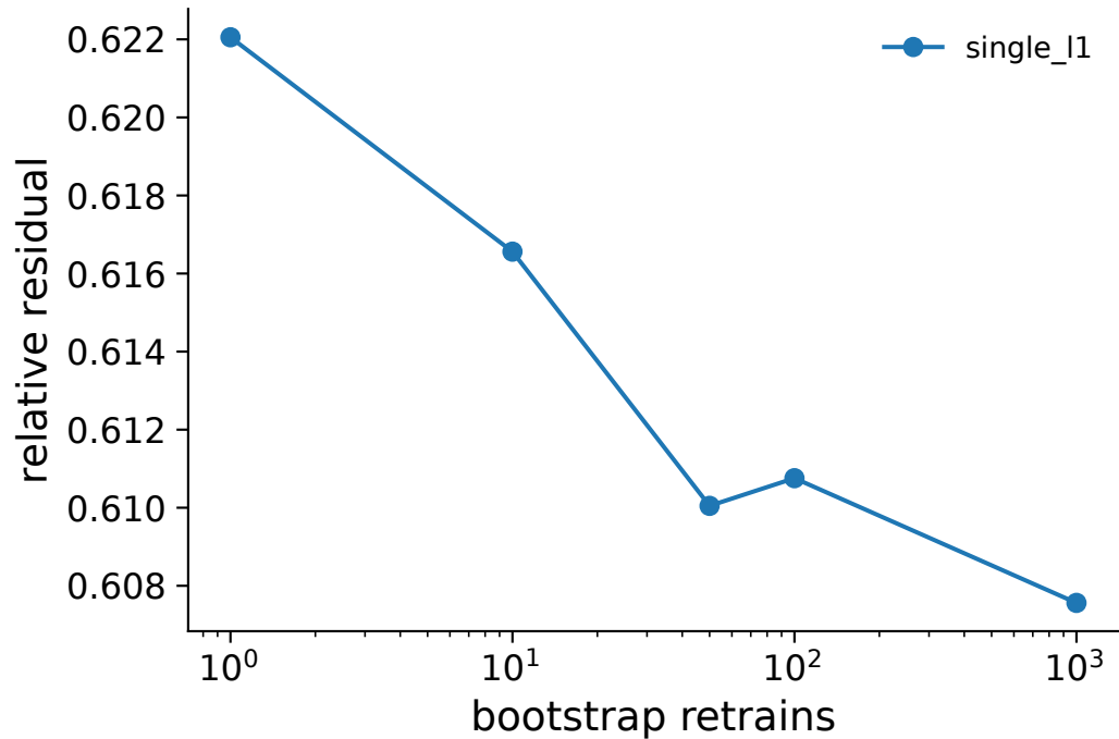
Relative Residual
