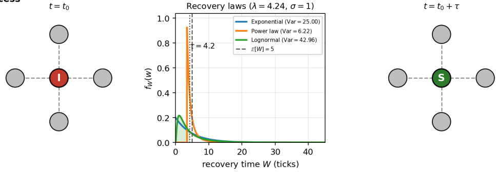
Figure 2: Grp-SIS schematic (after Tang et al., 2025, Fig. 1). (a) Memoryless infection per tick (probability \beta ). (b) Three recovery laws at common mean \mathbb{E}[W]=5 ticks: exponential, Tang power law, Tang lognormal.
