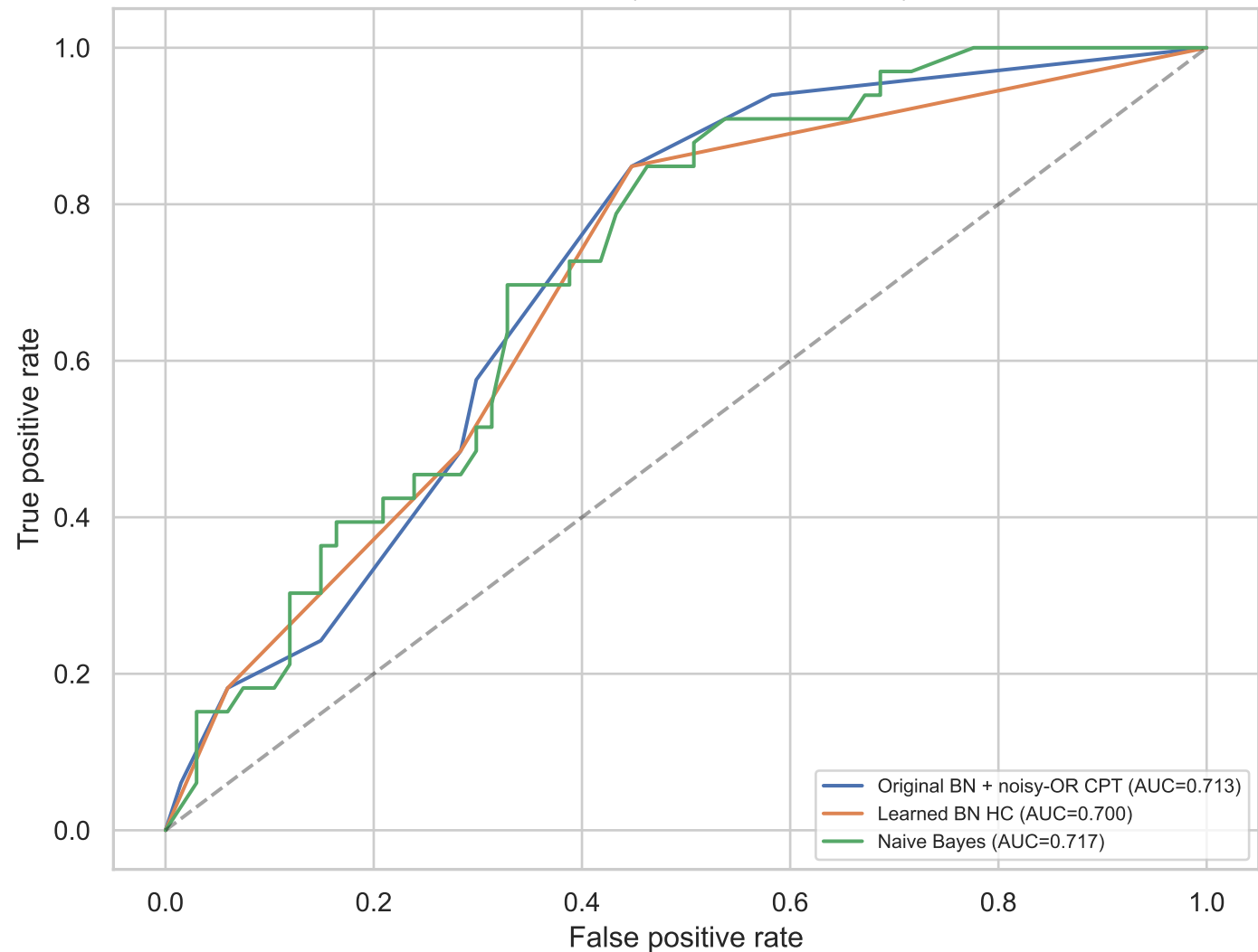
ROC curves (Train/Test = 100/100)
