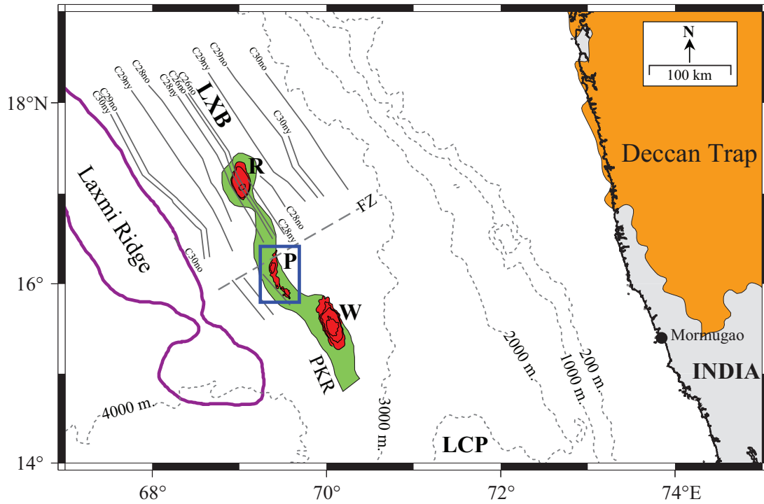
Figure 2: Generalized tectonic map of the northwestern continental margin of India and the adjoining deep ocean basins. The blue coloured box represents the study area. Grey coloured thin dotted lines represent the selected (200 m., 1000 m., 2000 m., 3000 m., and 4000 m.) bathymetry contours. Grey coloured continuous lines represent the inferred magnetic lineations in the Laxmi Basin (Bhattacharya & Yatheesh, 2015) and the solid red coloured patches in the axial part of the Laxmi Basin represent the extent of the seamount chain (Bhattacharya et al., 1994b) consisting of the Raman Seamount (R), Panikkar Seamount (P) and the Wadia Guyot (W). The green-coloured region represents the extent of the Panikkar Ridge (PKR). Other details are as in Figure 1.
