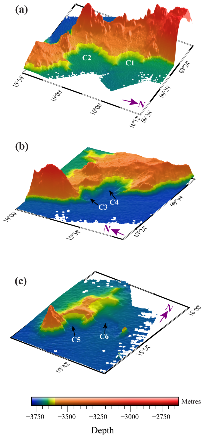
Figure 4: Colour-coded three-dimensional bathymetry maps representing postulated calderas (a) C1 and C2; (b) C3 and C4; and (c) C5 and C6. Other details are as in Figure 3.
