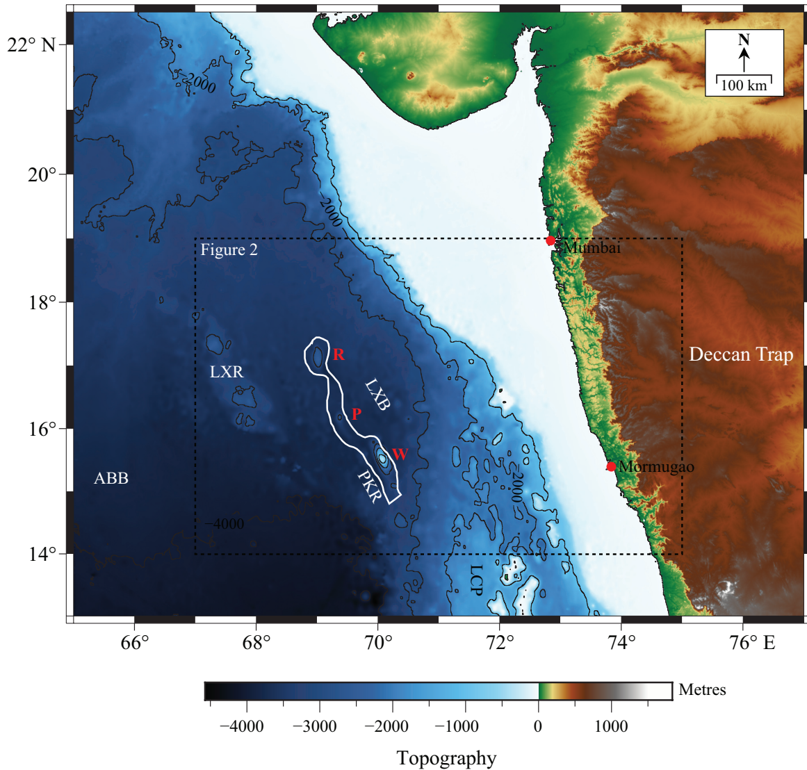
Figure 1: Topographic map of the northwestern continental margin of India and the adjoining deep oceans basins as depicted by the GEBCO 2021 global terrain model for ocean and land (GEBCO Compilation Group, 2021), showing the locations of the Panikkar Ridge (shown as thick white line) and the axial seamount chain in the Laxmi Basin. Thin black lines are selected (1000 m., 2000 m., 3000 m., and 4000 m.) bathymetry contours from GEBCO 2021 data set. The box shown with thick dashed black lines represents the boundary of the tectonic map shown in Figure 2. LXR: Laxmi Ridge; LXB: Laxmi Basin; ABB: Arabian Basin; PKR: Panikkar Ridge; LCP: Laccadive Plateau. R: Raman Seamount; P: Panikkar Seamount; W: Wadia Guyot.
