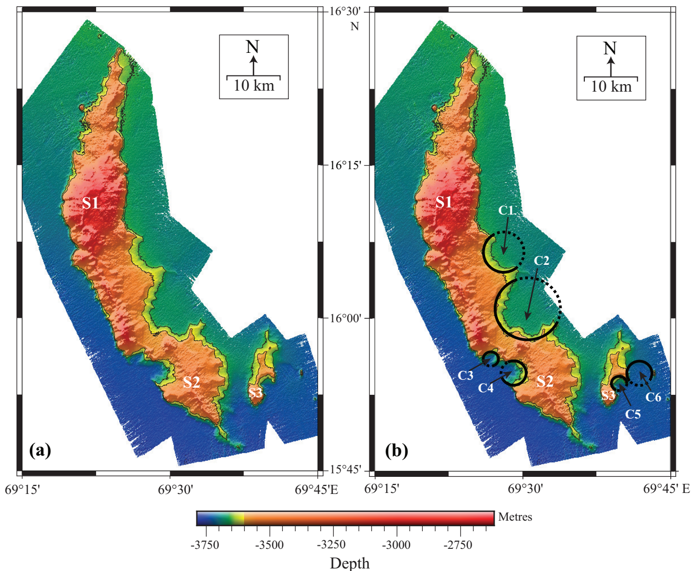
Figure 3: Colour-coded bathymetric map of the Panikkar Seamount and the adjacent regions, showing (a) the morphology of the seafloor and (b) the interpreted caldera-like features. The thin black lines represent selected (3600 m. and 3650 m.) isobaths. S1, S2 and S3 represent the Segment-1, Segment-2 and Segment-3 of the Panikkar Seamount. The labels C1 through C6 represent the locations of inferred caldera-like features. The thick black circles represent the postulated extent of rims of these inferred calderas as seen from the bathymetry data (continuous semi-circles) and as considered to have buried under the sediments (dotted semi-circles).
