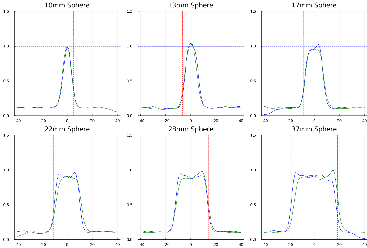
Figure 2: Intensity Profiles for Spheres (Relative RC). The x-axis represents the distance from the sphere center in millimeters (mm).
