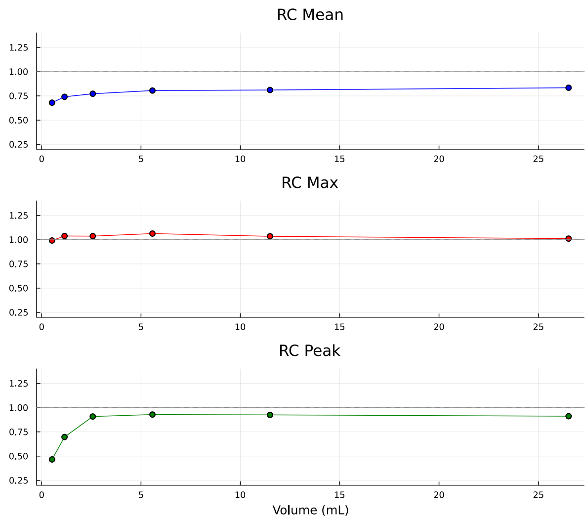
Figure 3: Recovery Coefficient curves
