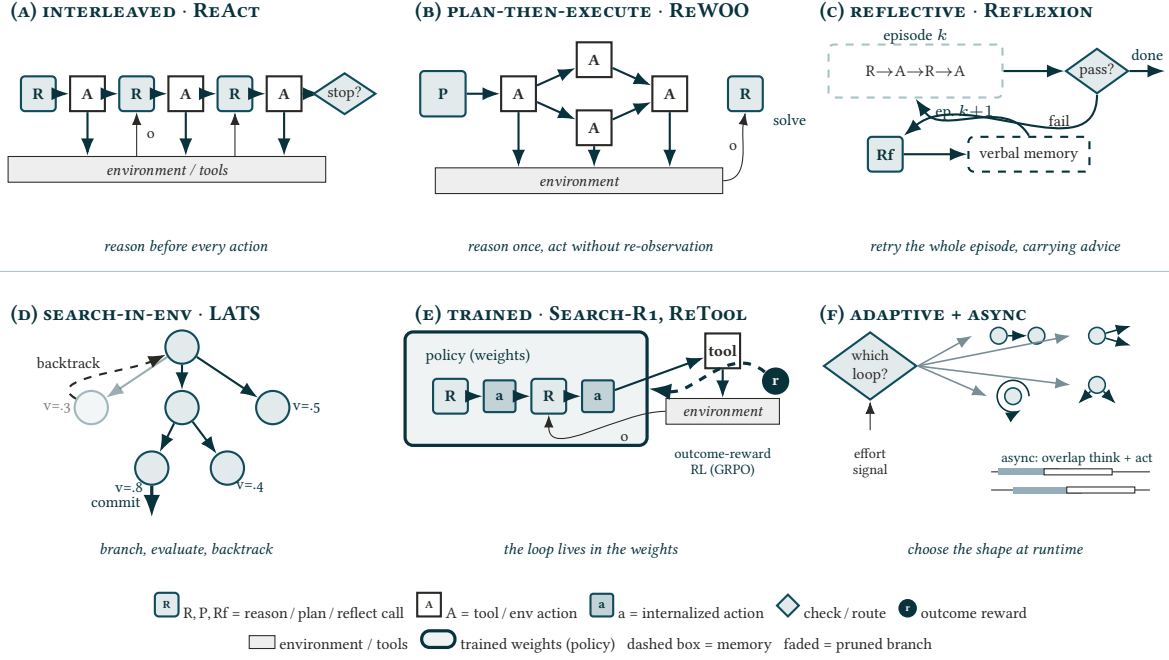
FIGURE 4: The loop zoo: six loop shapes drawn on one shared notation (legend at bottom). (a) Interleaved reasoning and action reasons before every step (Yao et al. 2022). (b) Plan-then-execute produces one up-front plan, executed without re-observation, optionally as a parallel DAG (Xu et al. 2023; Kim et al. 2023). (c) Reflective loops convert a failed episode into stored verbal advice and retry the whole episode (Shinn et al. 2023). (d) Search-in-environment branches, evaluates, and backtracks (Zhou et al. 2024a). (e) Trained loops absorb the same interleaved cycle into the weights and optimize it against outcome reward (Jin et al. 2025; Feng et al. 2025a). (f) Adaptive and asynchronous loops let a controller pick the shape at runtime and overlap thinking with acting (Sun et al. 2023; Paglieri et al. 2025; Ginart et al. 2024). Shapes (b) through (f) are each a relaxation of (a)’s reason-before-every-step default; what each relaxation assumes and costs is Table 2.
