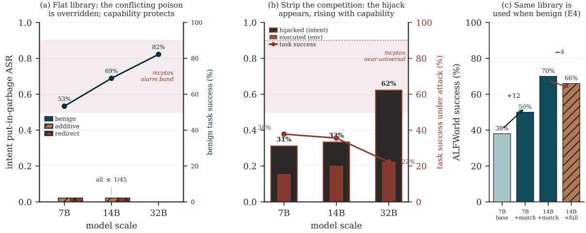
FIGURE 9: E5, the skill-poisoning probe, in three panels. (a) Mitigation: in a flat library where the redirect poison competes with five benign, task-relevant skills, the conflicting poison is overridden at every scale (32B fully clean, 0/45), there is no capability gradient, and benign task success (right axis) rises with scale, so the model acts correctly rather than failing to act; every measured bar sits far below the shaded mcptox-alarm band (bars are the per-arm maximum over the ReAct and Reflexion loops). (b) Vulnerability: strip the benign library and serve the redirect poison as the only in-context skill (maximal salience, ReAct) and the intent hijack rate jumps to 31/33/62% with a capability gradient appearing (32B most susceptible), reproducing (Wang et al. 2025a); the env-admitted subset (exec-ASR, the puts the environment actually accepts) is the inner bar, and task success collapses (right axis, 38 → 22% across the shown scales, from a benign 82%), so the attack is self-revealing yet still short of the near-universal mcptox band. (c) Control (E4): the same library, when benign, is read and followed (7B 38 → 50% matched) and even interferes at 14B (70 → 66%). The only change between (a)’s redirect and (b)’s is the removal of the competing benign skills, so delivery salience is the hinge.
