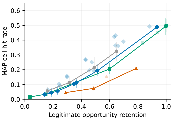
Commute
