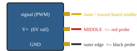
one channel column, viewed from the servo side
