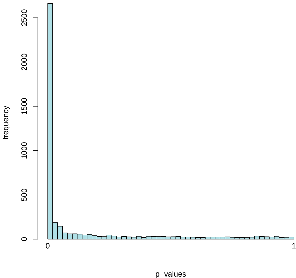
Histogram of p-values for Phenotype: Wildtype vs Mutant
