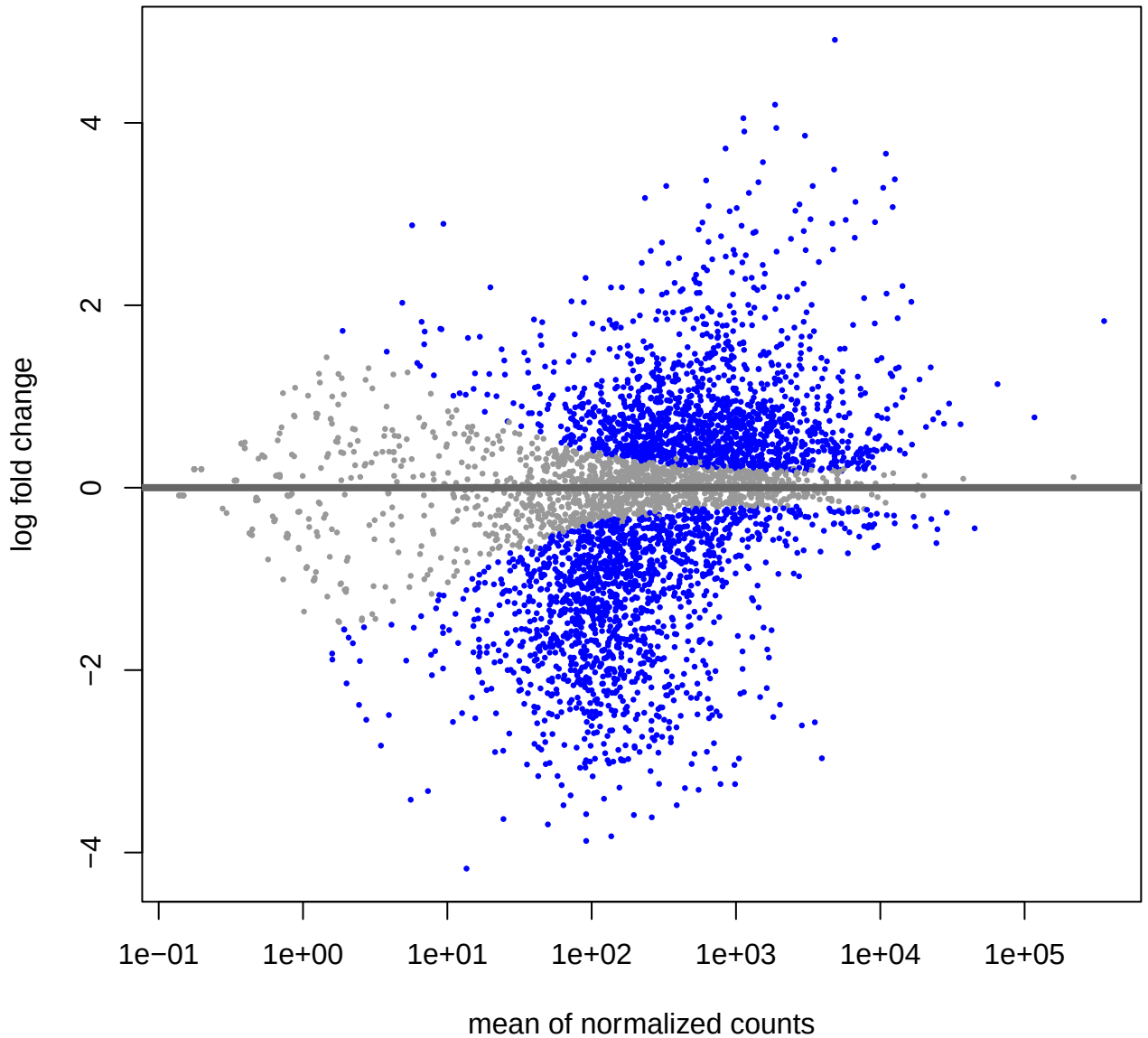
MA-plot for Phenotype: Wildtype vs Mutant
