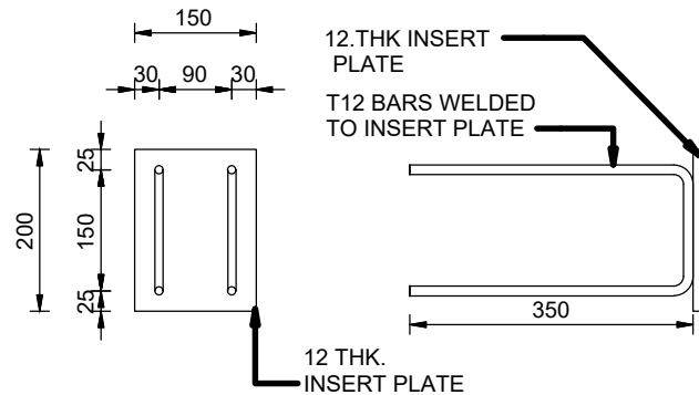
DETAILS OF INSERT PLATE IP1
