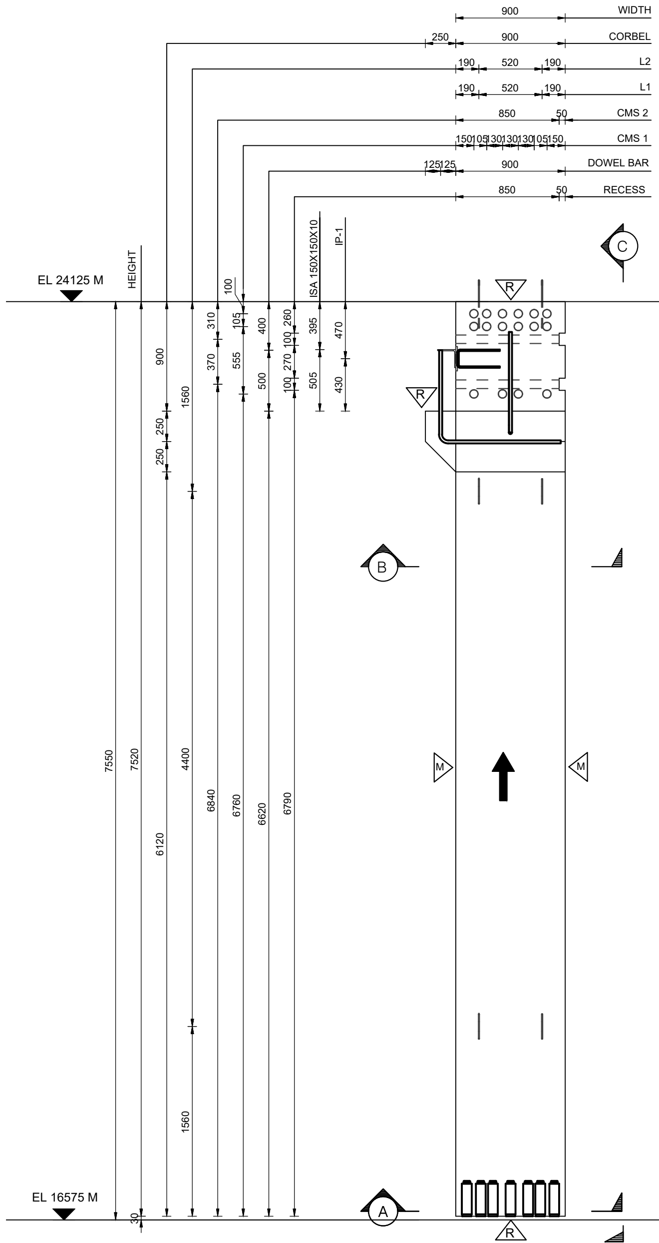
DETAILS OF PRECAST COLUMN SCALE = 1 : 30
