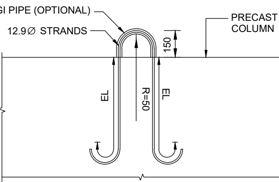
TYPICAL LIFTER DETAIL
