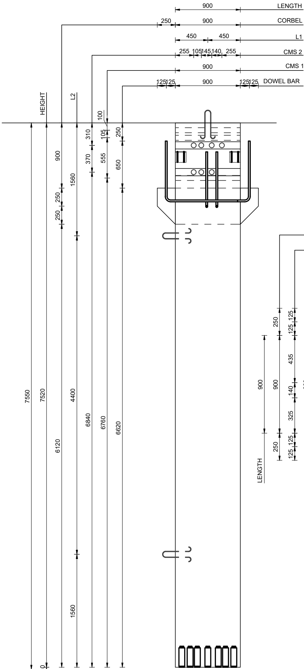
ELEVATION C SCALE - 1 : 30
