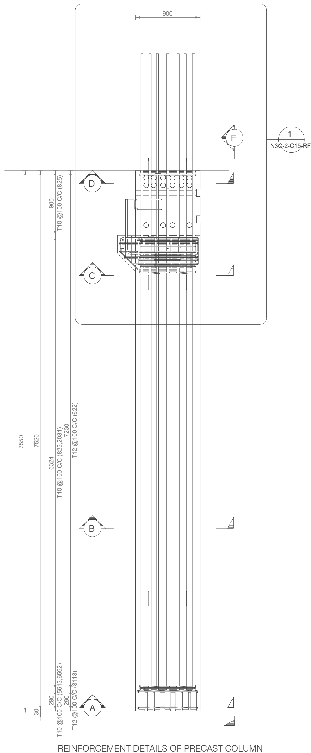
REINFORCEMENT DETAILS OF PRECAST COLUMN
