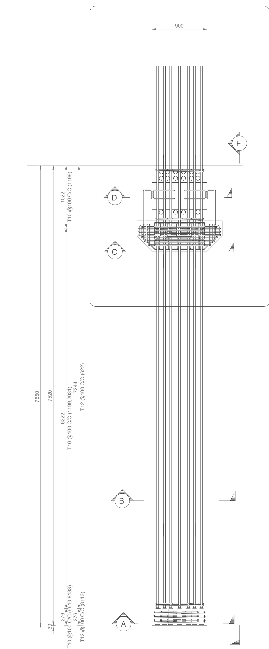
REINFORCEMENT DETAILS OF PRECAST COLUMN SCALE = 1 : 30
