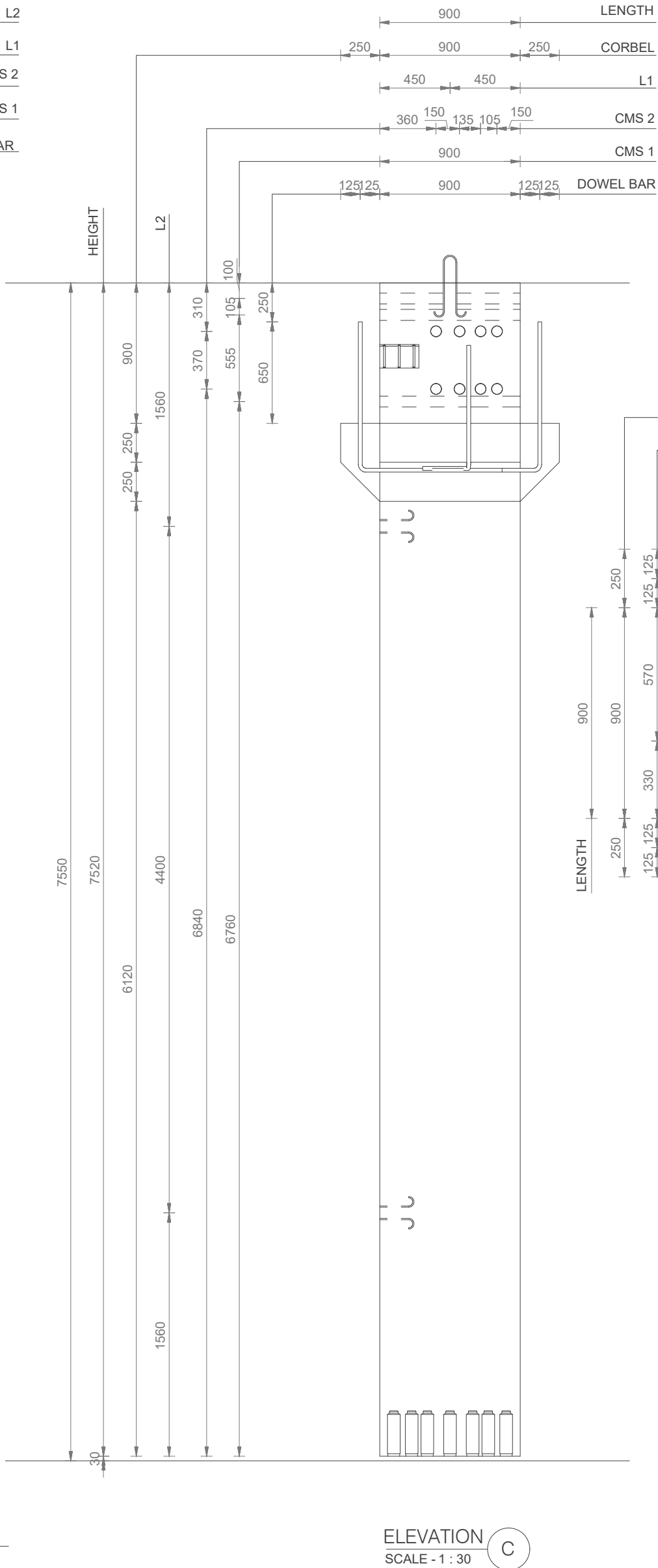
DETAIL OF PRECAST COLUMN SCALE = 1 : 30
