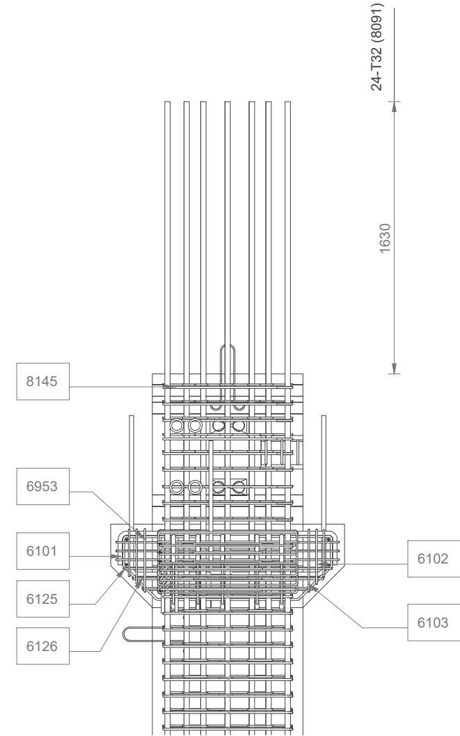
DETAIL SCALE - 1 : 30
