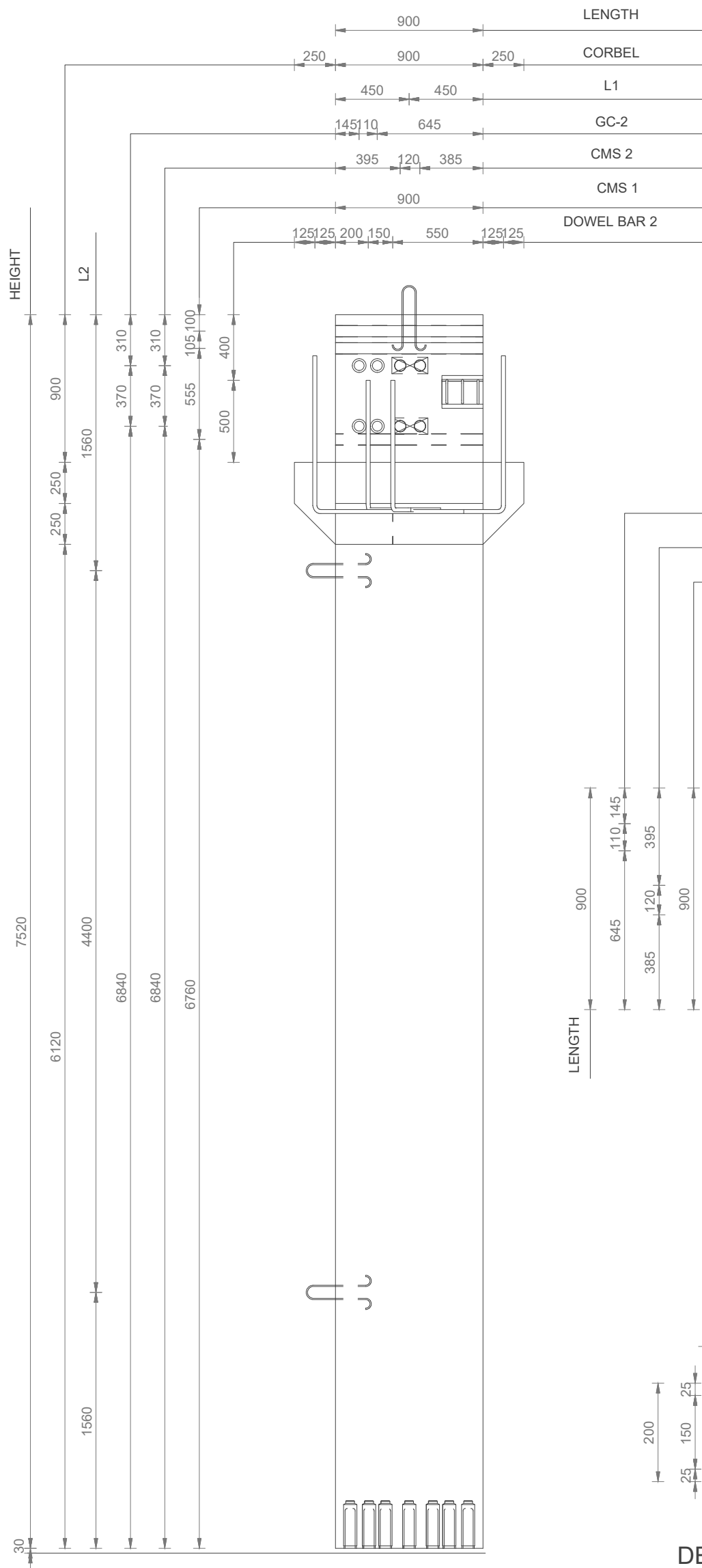
ELEVATION SCALE - 1 : 30
