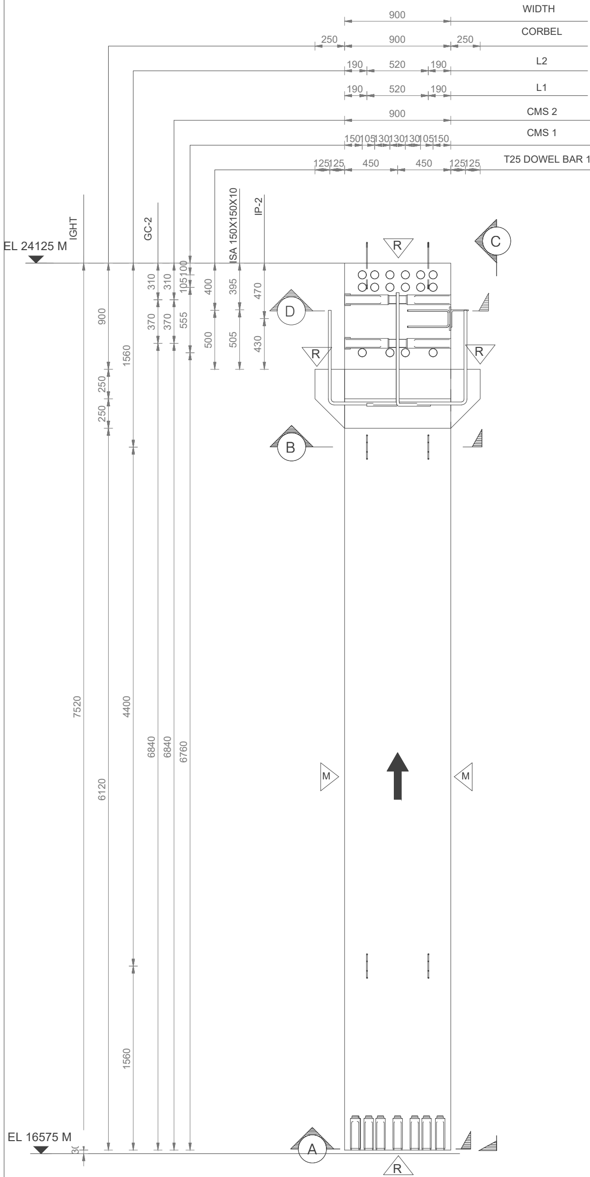
DETAILS OF PRECAST COLUMN SCALE = 1 : 30
