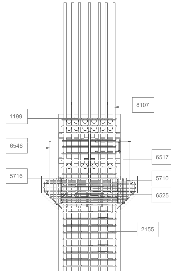
DETAIL SCALE - 1 : 30
