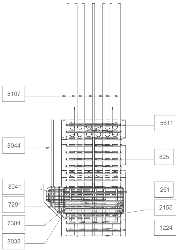
DETAIL SCALE - 1 : 30
