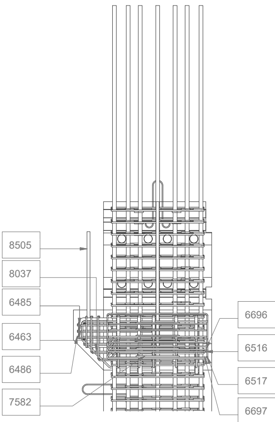
DETAIL SCALE - 1 : 30
