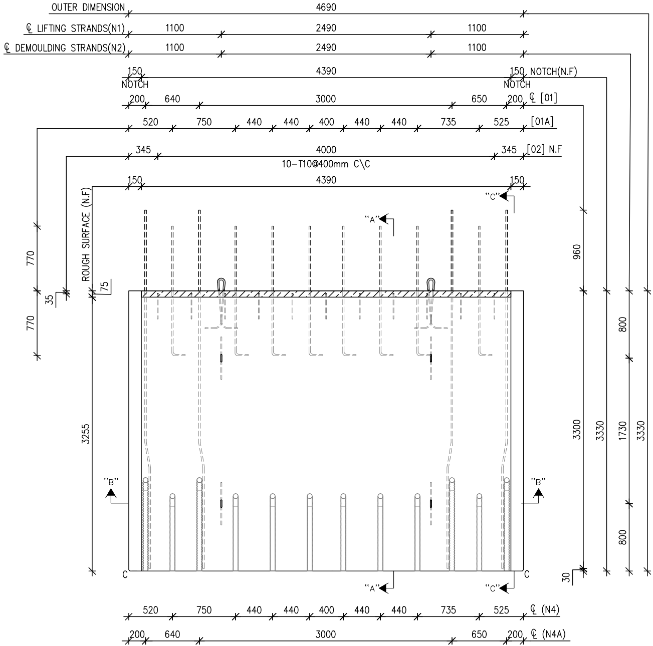
PLAN VIEW (1:45)
