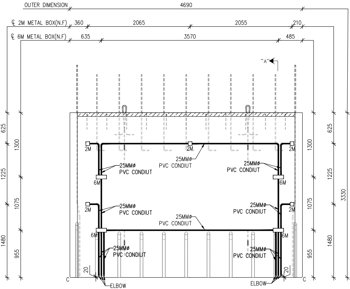
PLAN VIEW (1:45)
