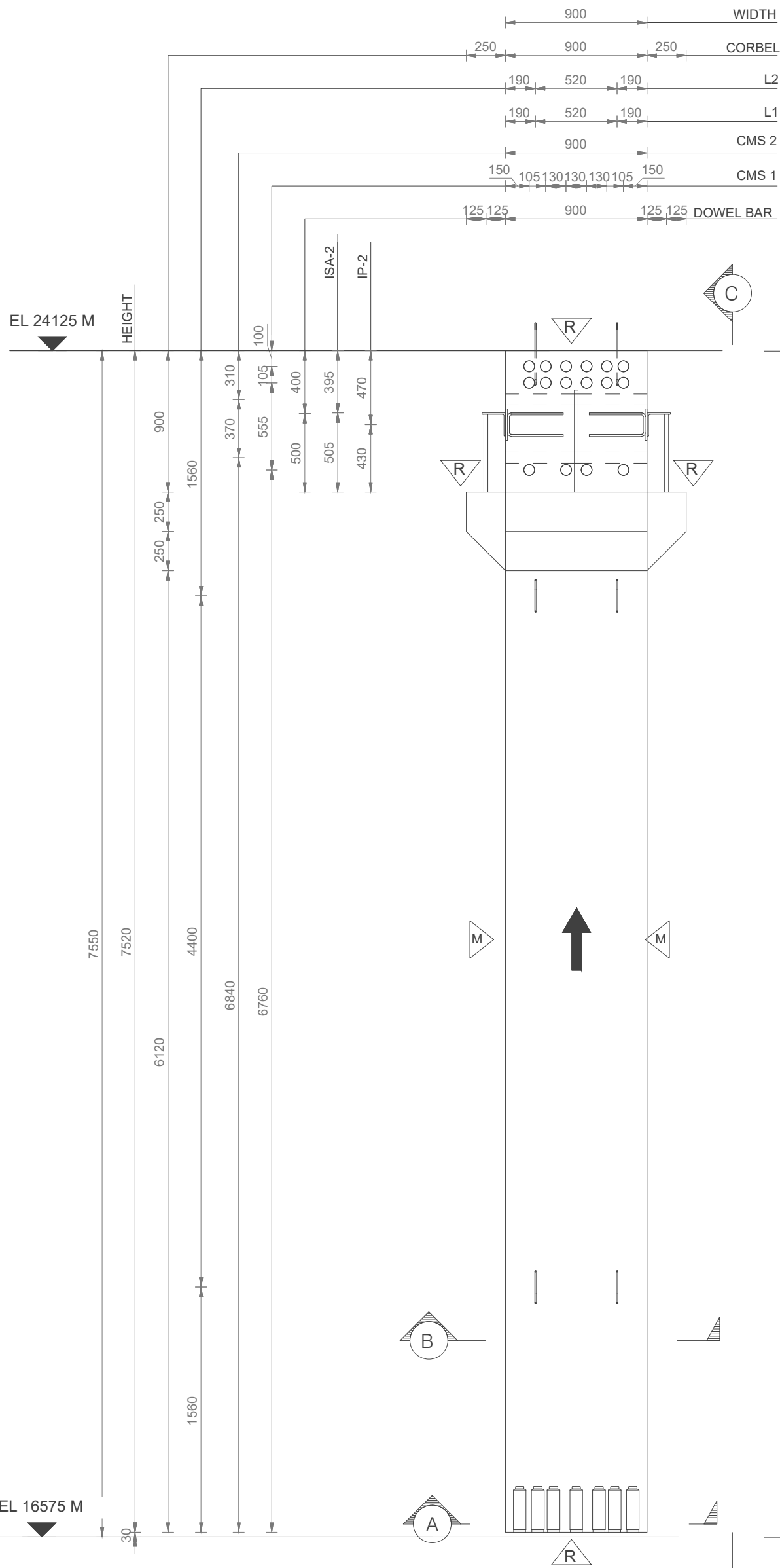
DETAIL OF PRECAST COLUMN SCALE = 1 : 30
