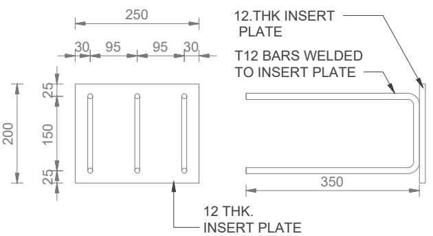
DETAILS OF INSERT PLATE IP2
