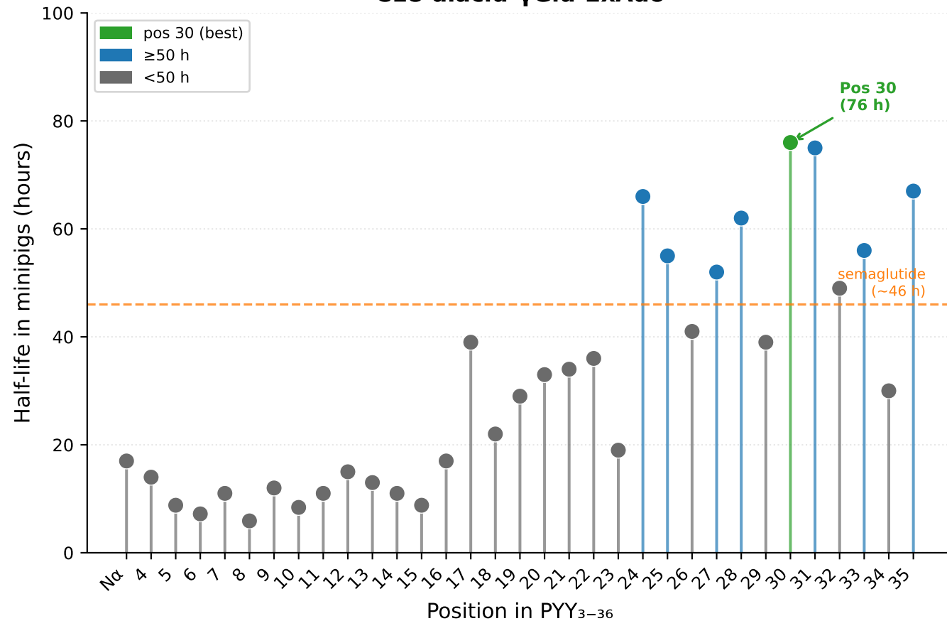
(a) Half-life vs. lipitation position C18 diacid- \gamma Glu-2xAdo
