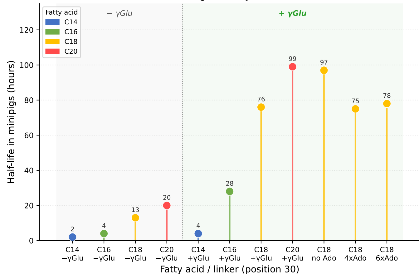
(b) Half-life vs. fatty acid length \pm \gamma Glu all analogues at position 30
