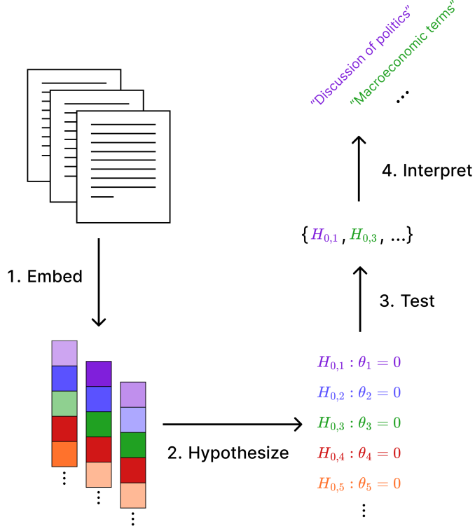
Figure 1: The proposed framework for discovery from unstructured data.
